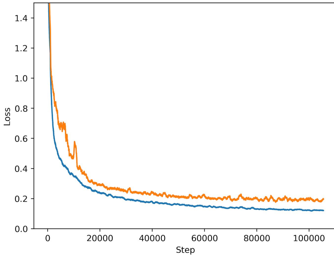
Supplemental Figure 3. Learning curves for deep learning model. The summed combined loss for binary cross entropy classification and 9 value regressions of the three circles (center coordinates and radii) are shown against the iterations. The training loss is shown in blue and the validation loss is shown in orange.
