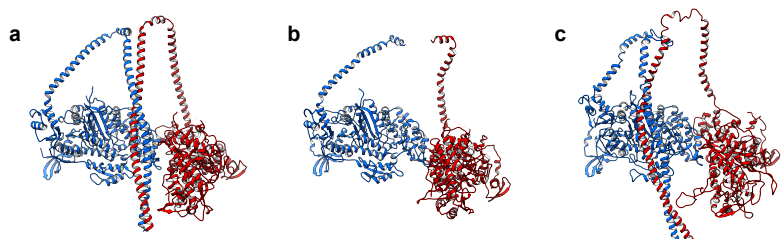
a Shutdown SmM (present study) b SmM HMM - 1184 c Tarantula IHM - 3JBH
