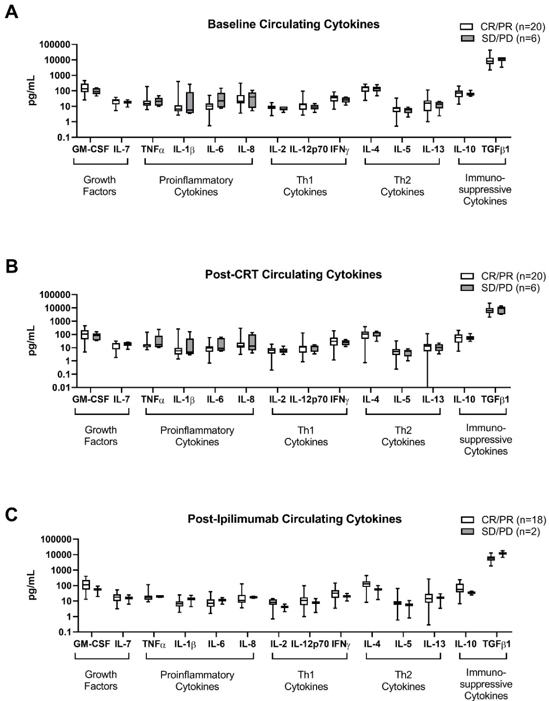
Supplemental Figure S6. Association of circulating cytokine levels with objective clinical response. Circulating plasma cytokines were measured from blood collected at (A) baseline, (B) post-CRT, and (C) post-ipilimumab using a multiplexing bead-based immunoassay. Levels of cytokines were correlated with overall clinical response. Box-plots show 25 th to 75 th percentiles with median value indicated by horizontal line. Whiskers indicate minimum and maximum values. CR= complete response; PR= partial response; SD= stable disease; PD=progressive disease. All comparisons were non-significant.
