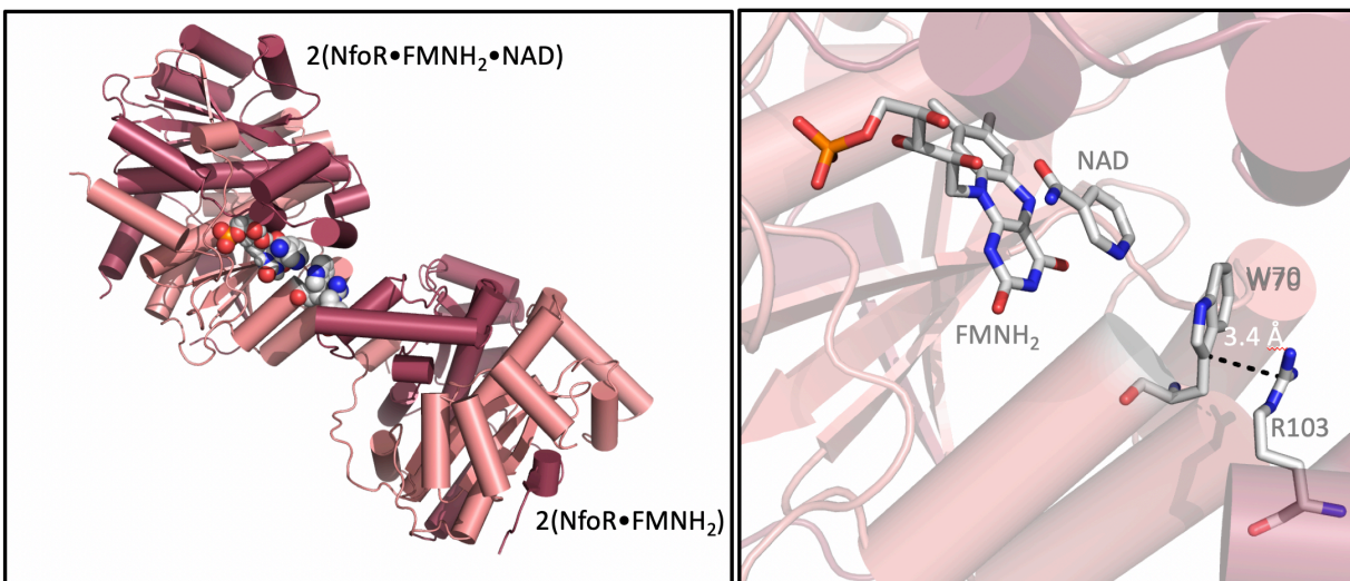
Figure S1. Binding of the Nicotinamide Ring of NAD + is a crystal soaking artifact The nicotinamide is stabilized by close \pi - \pi / \pi -cation stacking of W70 and R103 across the crystallographic contact.
