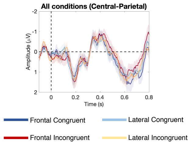
Figure S1: ERPs at the onset of the non-critical word, averaged from nine central-parietal electrodes (C1, Cz, C2, CP1, CP1, CPz, CP2, P1, Pz, P2), for all experimental conditions.
