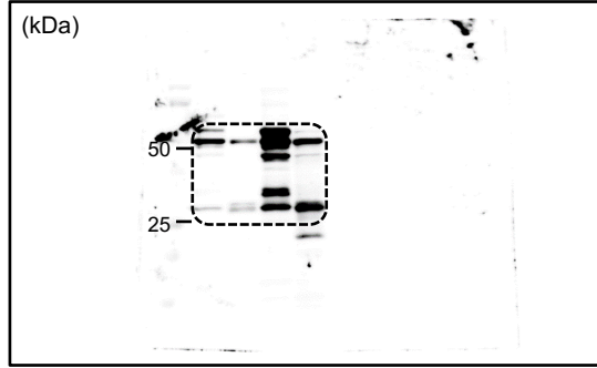
Blot: anti-FTMT
