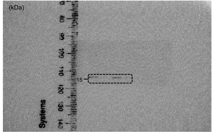
Blot: anti-LC3
