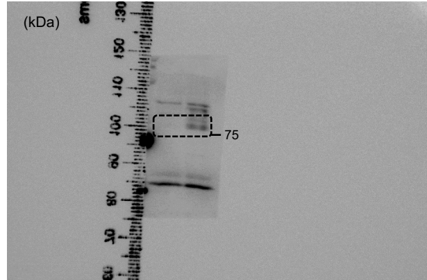
Blot: anti-FTMT
