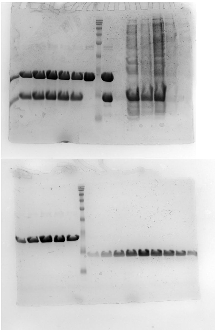
Original gel pictures for Figure 6E (SiaB/SiaC complex).
