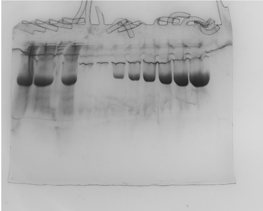
Original gel picture for Figure 6E (SiaB/SiaC complex dissociation) with annotation. The area in red rectangle was cropped out for publication.
