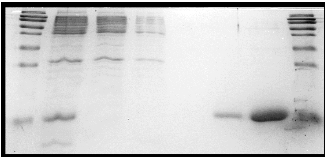
Original gel picture for Figure S2B (purification of SiaC P )
