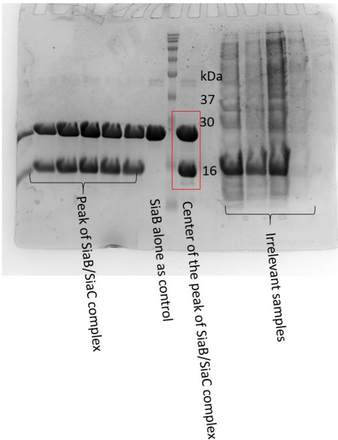
Original gel pictures for Figure 6E (Siab/Siac complex) with annotation. The area in red rectangle was cropped out for publication.
