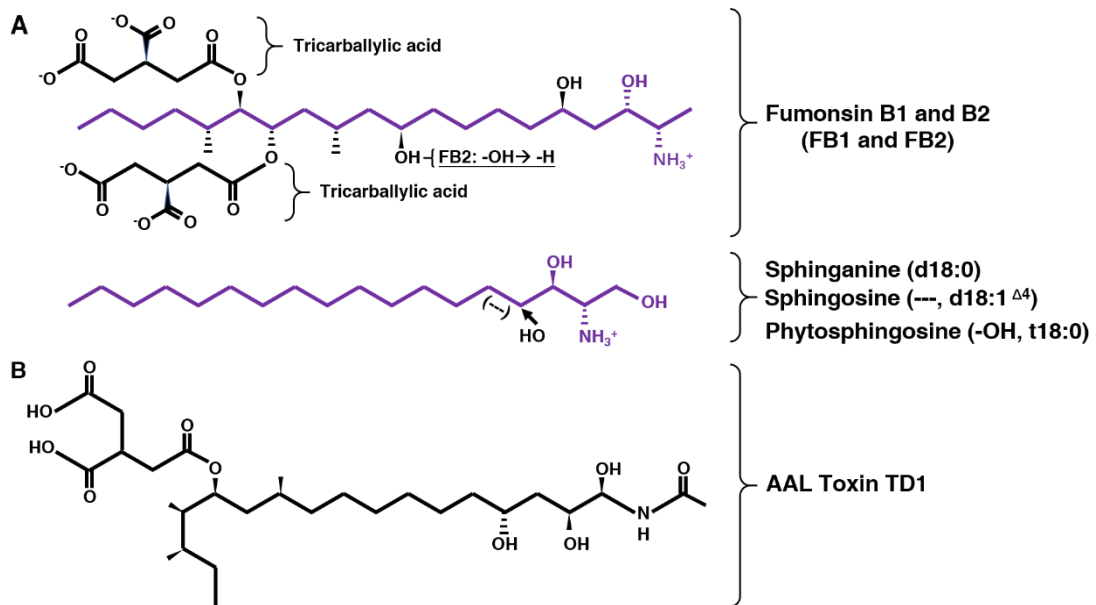
Supplemental Figure S1. Structures of major fumonisins, representative LCBs and AAL toxin.
