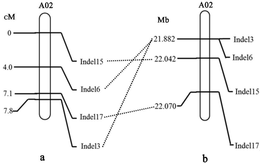
Additional file 4: Figure S2 The local genetic linkage map and physical map of cqSPDA2 on chromosome A02 in BC 3 F 2 population. a The local genetic linkage map. b The physical map.
