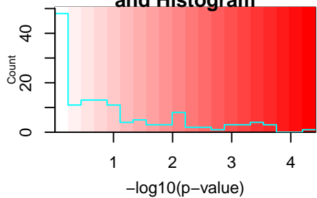
Color Key and Histogram
