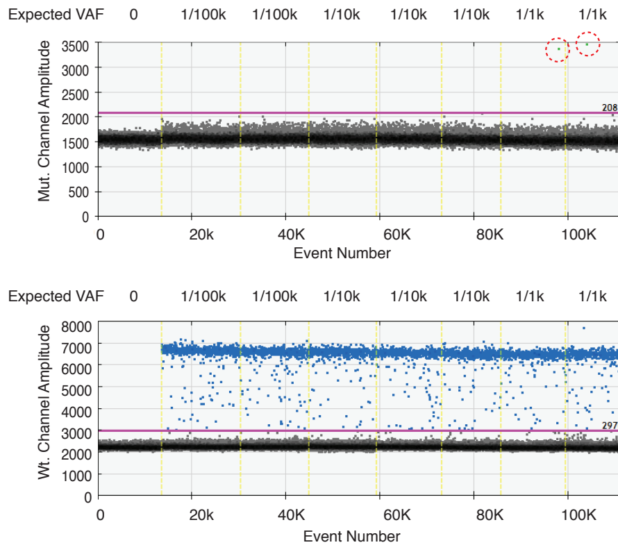
Supplementary Figure 4: Digital droplet PCR (ddPCR) testing for single mutation in dilution series. (A) The observed VAFs of HapMap serial dilutions measured by using a ddPCR assay for a single mutation (with three replicates) vs. the expected VAFs; (B) The representative ddPCR raw data and fluorescence intensity thresholds for determining positive or negative droplets.
