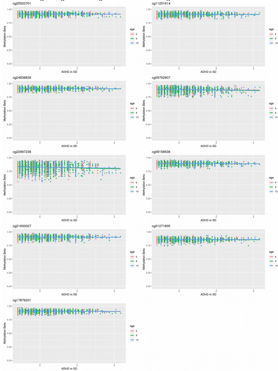
Figure S2: Scatterplot of genome-wide significant CpG sites (birth methylation EWAS) in the Generation R Study. Red indicates ADHD levels at age 6, green at age 8 and blue at age 10.
