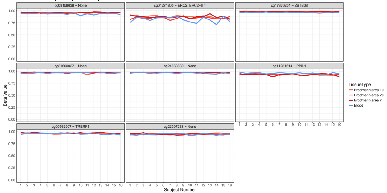
Figure S1: Methylation levels of genome-wide significant CpG sites (cord blood EWAS) in brain and blood tissue of 16 participants in the BECon database.
