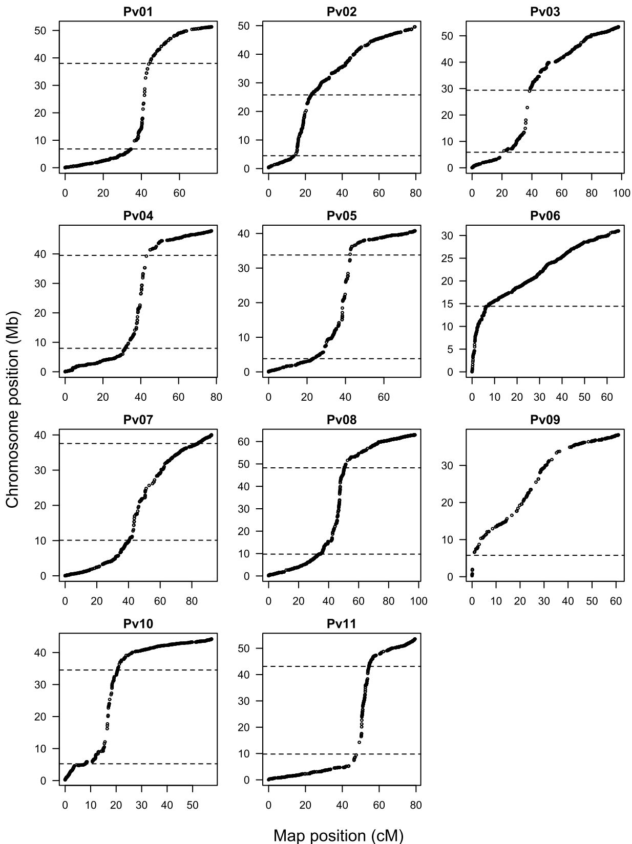
Additional file 8. Comparison between the physical location and the recombination frequency (genetic map position) based on thinned GBS markers (5.738 markers). The dashed horizontal lines represent the boundaries for the pericentromeric regions as defined by Schmutz et al. (2014).
