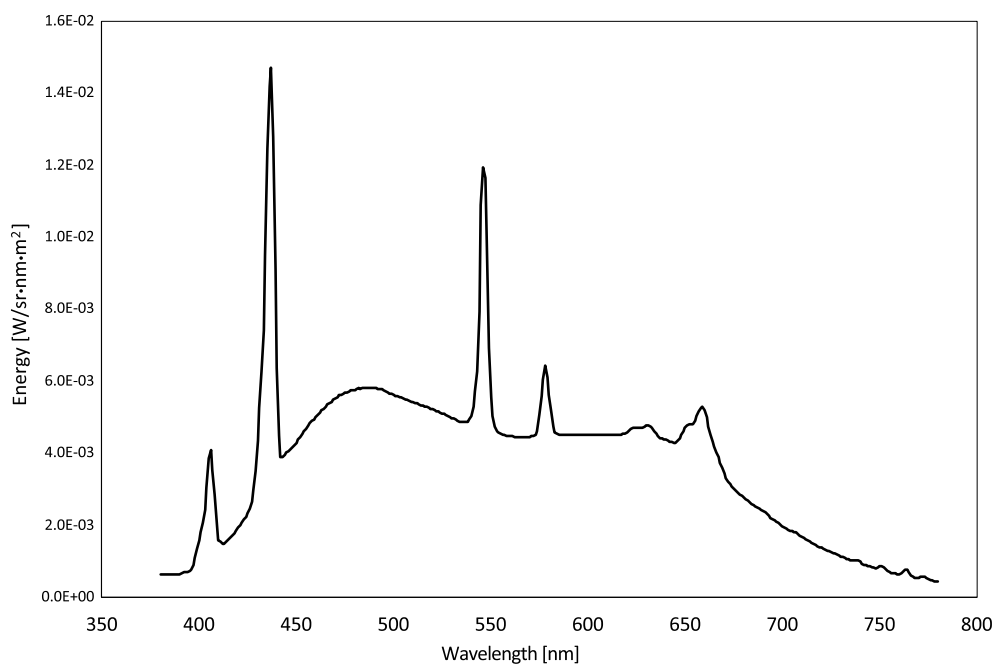
Supplementary Figure S1. Energy spectrum of VeriVide65 lamp used in the experiment.
