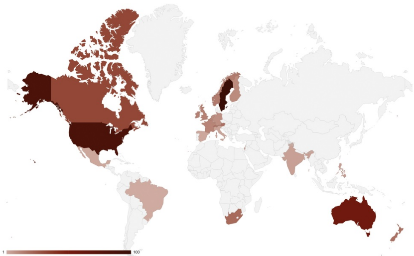
Figure E1 Global heat map of relative search volume (RSV) for "Alpha-gal allergy" (topic), 2004-2019. Highest RSV was in the following countries: Sweden, United States, Canada, Australia, and South Africa.
