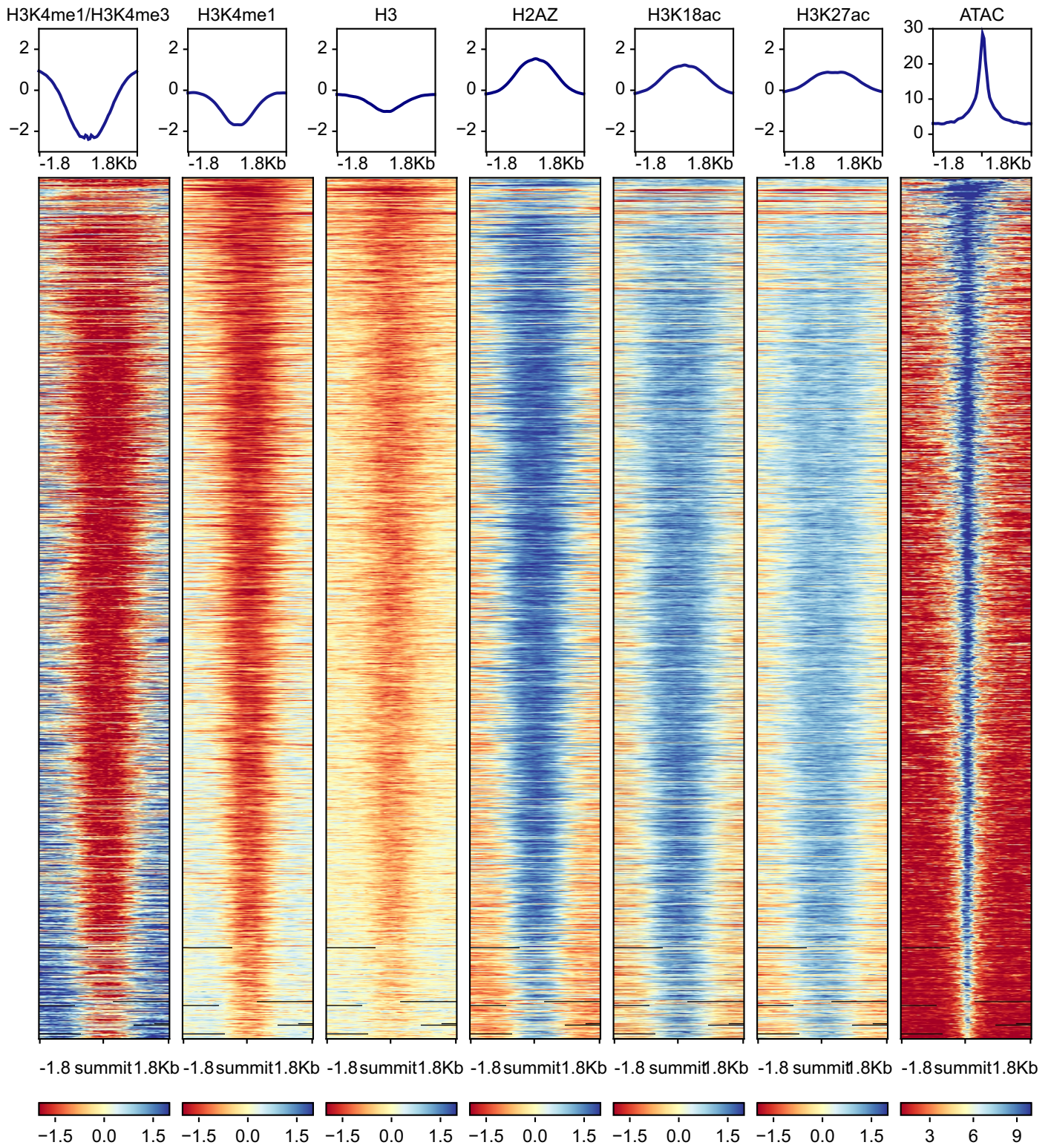
Schizont stage ATACseq peak summits
