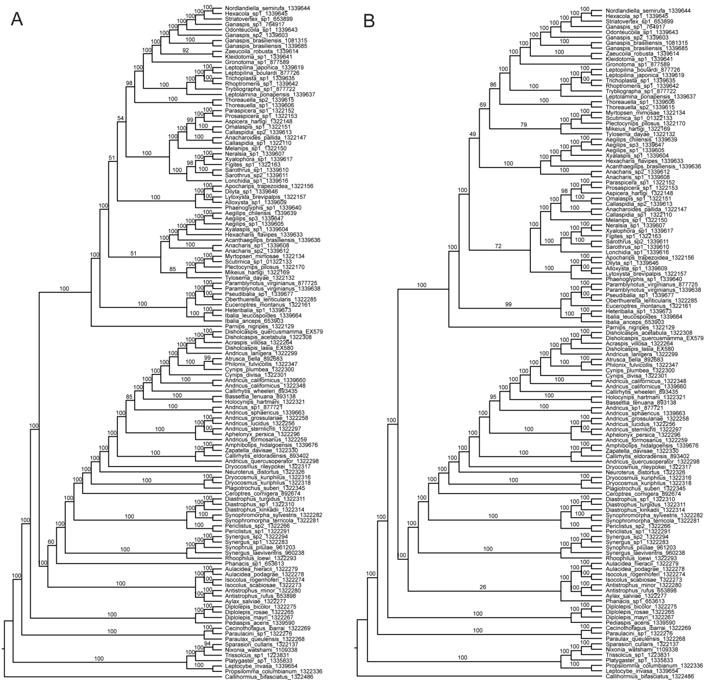
Additional file 11: Additional trees estimated while excluding Eschatocerus niger . All trees are presented as cladograms for clarity of relationships, and are based on a combined ML search for the best tree and 1000 bootstrap replicates using unpartitioned data matrices. Bootstrap support values are displayed next to respective nodes. Analyses were rooted using the outer outgroup Callihormius bifasciatus . A) 50% completeness matrix, B) 70% completeness matrix.
