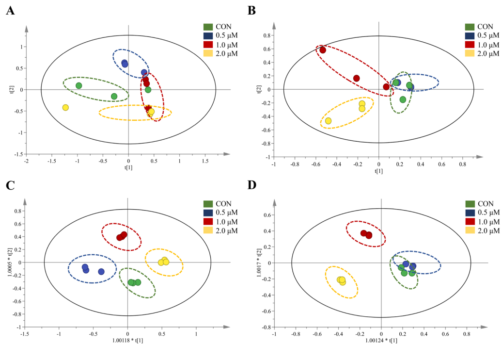
Figure S1. Scores plots of PCA and OPLS-DA from cellular metabolomics. (A) Scores plot of PCA in positive mode. (B) Scores plot of PCA in negative mode. (C) Scores plot of OPLS-DA in positive mode. (D) Scores plot of OPLS-DA in negative mode.
