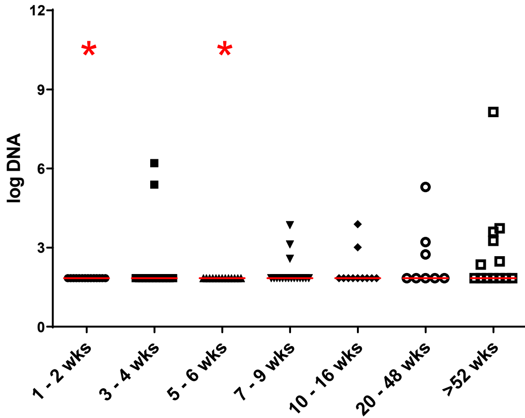
Supplemental Figure 2. Abundance (log DNA) of Clostridium perfringens enterotoxin gene. Red lines indicate medians and red asterisks indicate significance in comparison to adult dogs (i.e., dogs > 52 weeks of age; p < .05 ).
