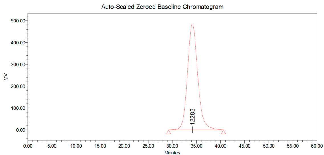
Figure S2. The elugram obtained from SEC for PSF sample.
