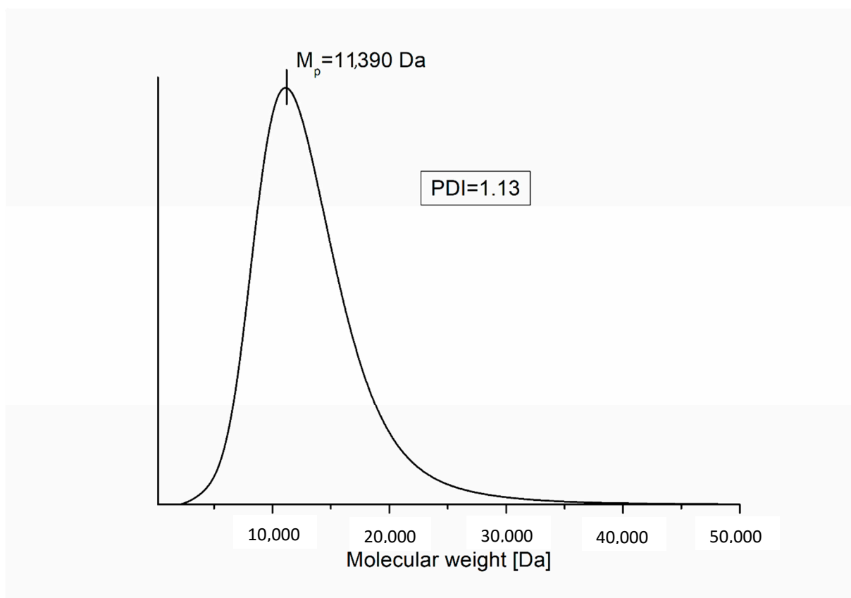
Figure S3. The molecular weights distribution in the sample PSF determined on the base of SEC analyses.
