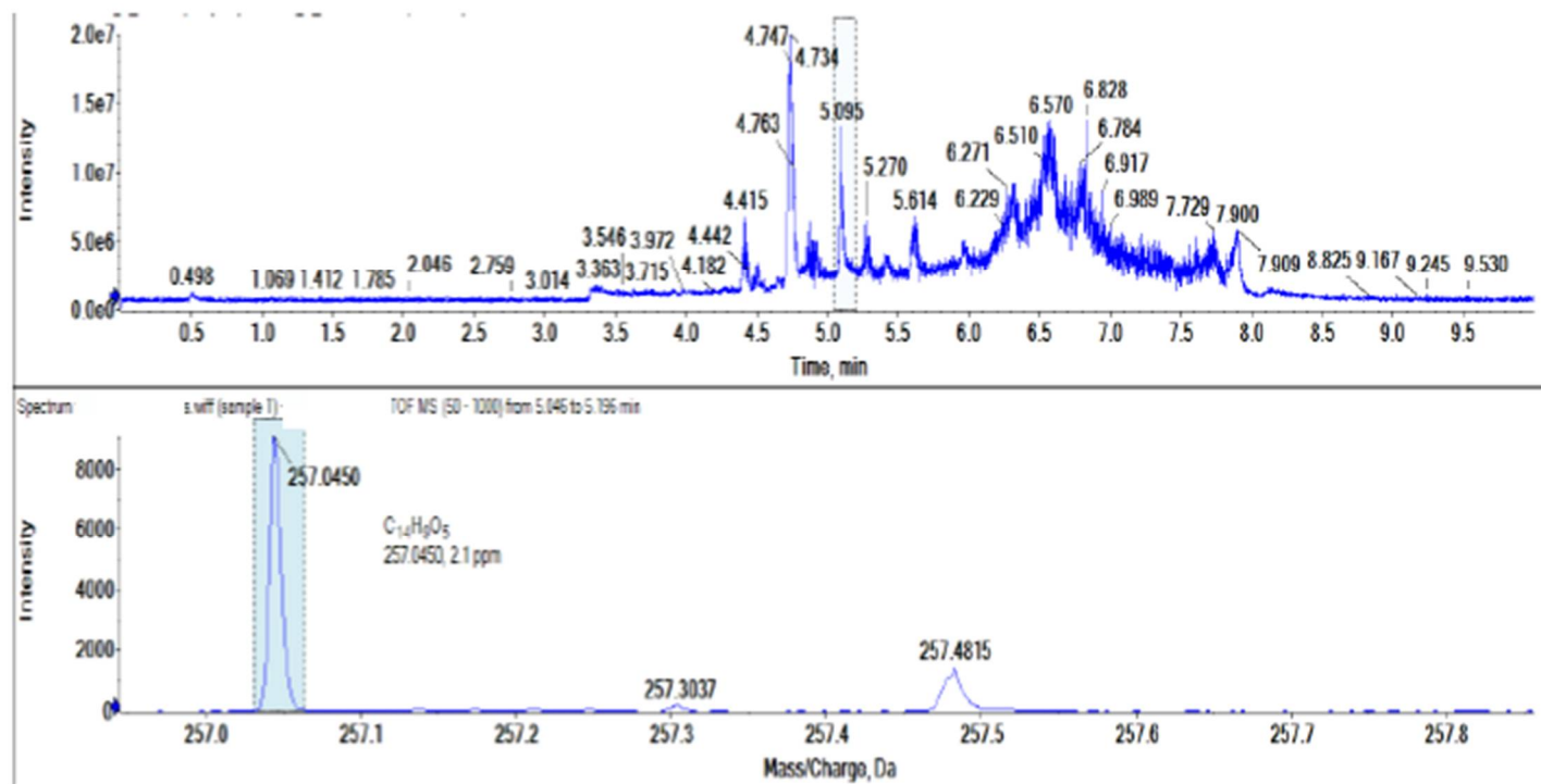
Page S23: Figure S21. HRESIMS spectrum of muracatane B (3).
