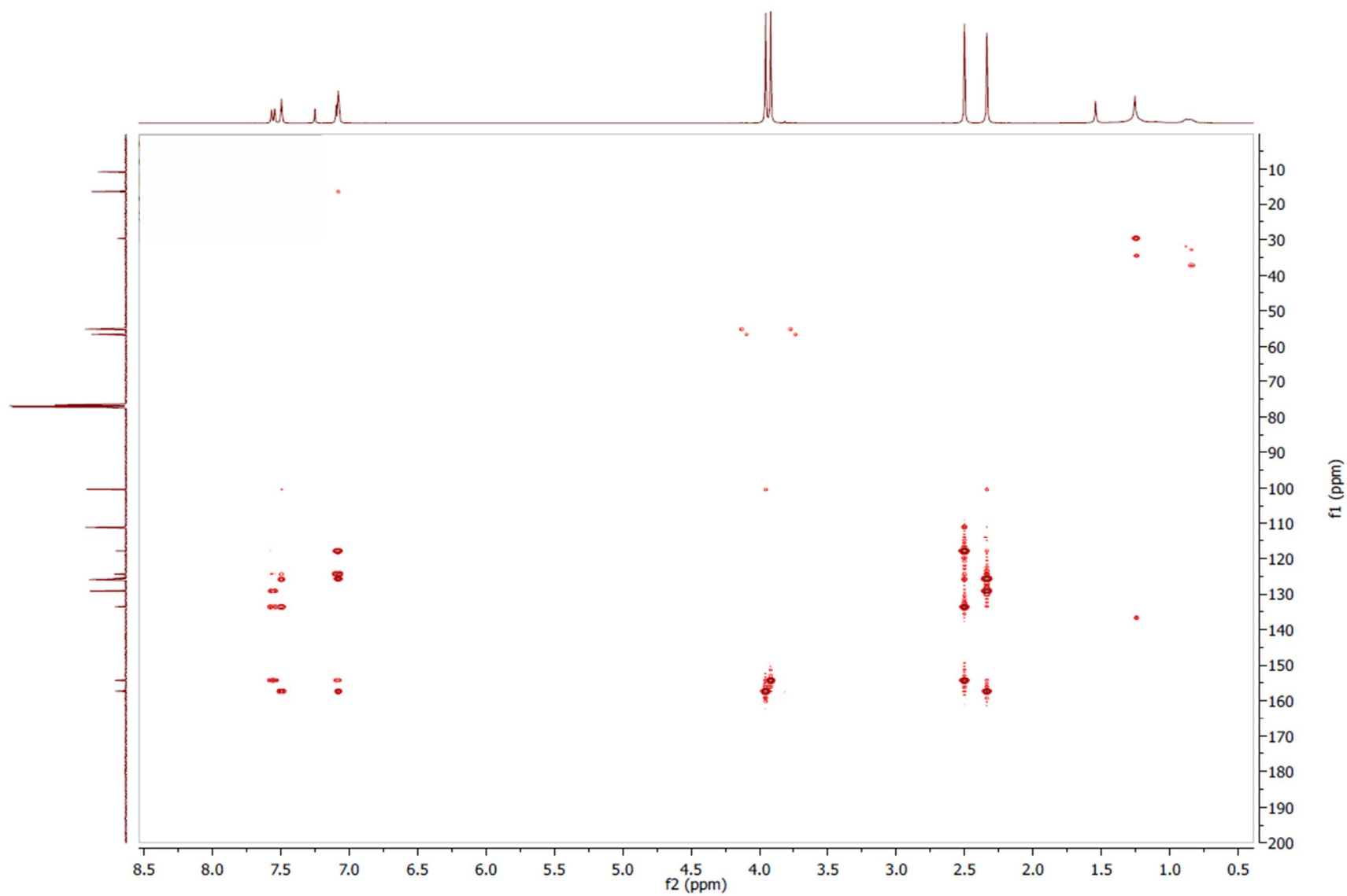
Page S29: Figure S27. HMBC spectrum of muracatane C (4) (400 MHz, CDCl 3 ).
