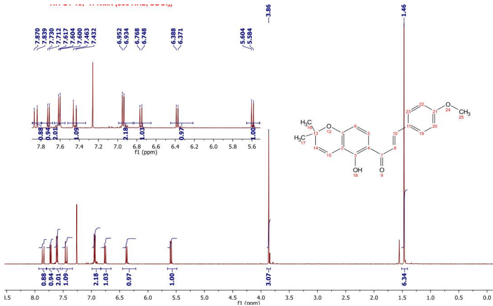
Page S31: Figure S29. 1 H NMR spectrum of 4-methoxylonchocarpin (5)
