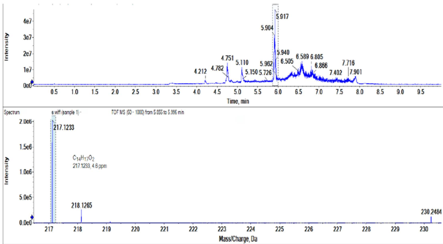
Page S30: Figure S28. HRESIMS spectrum of muracatane C (4).
