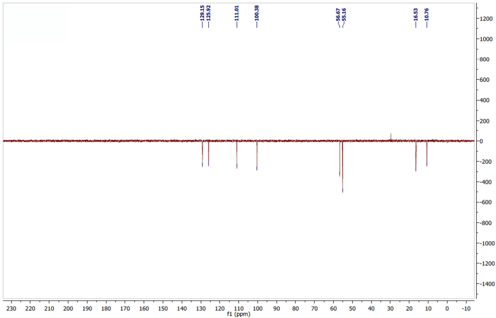
Page S26: Figure S24. DEPT spectrum of muracatane C (4) (400 MHz, CDCl 3 ).
