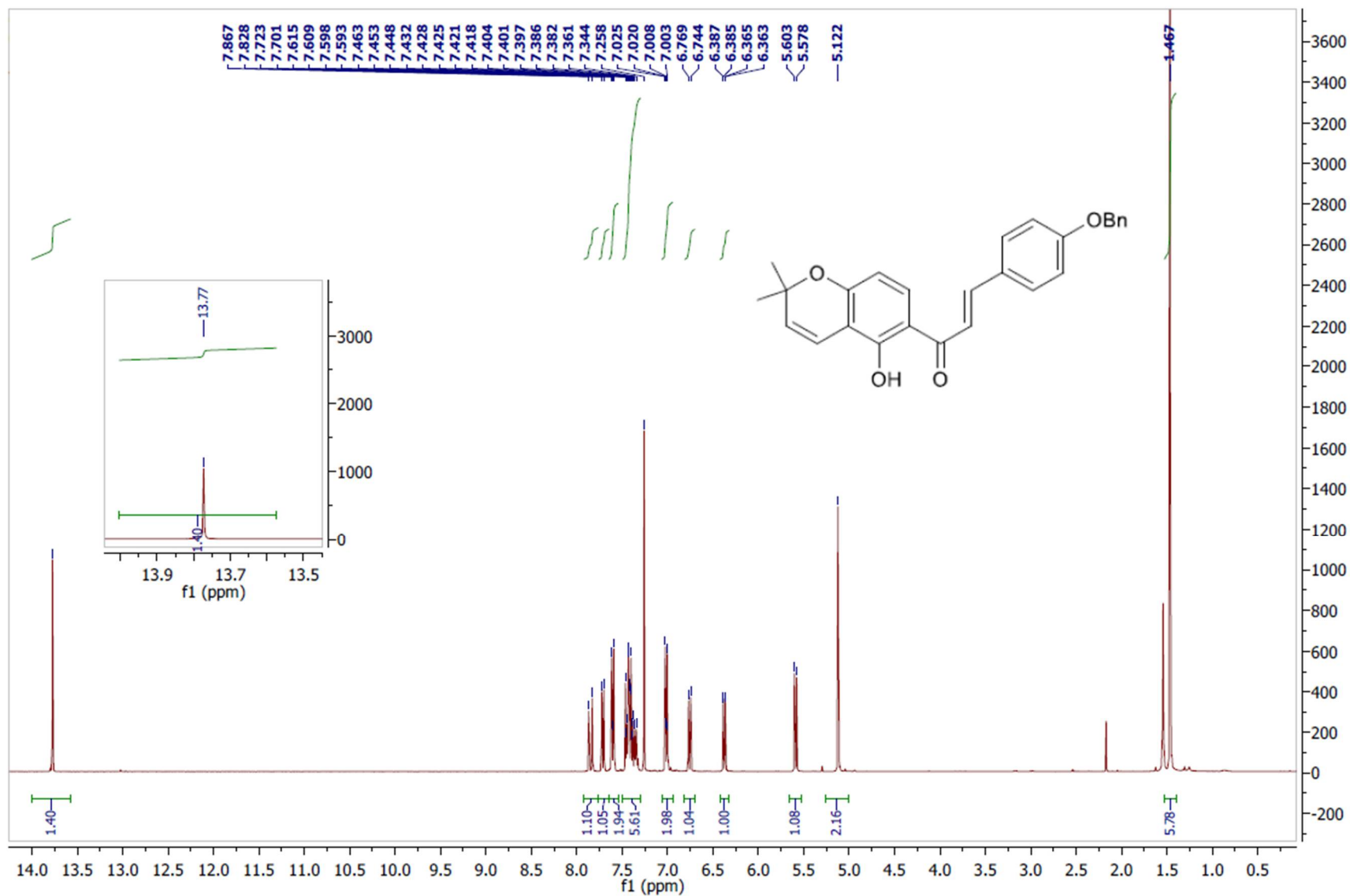
Page S5: Figure S3. 1 H NMR spectrum of 4-benzyloxylonchocarpin (1) (400 MHz, CDCl 3 ).
