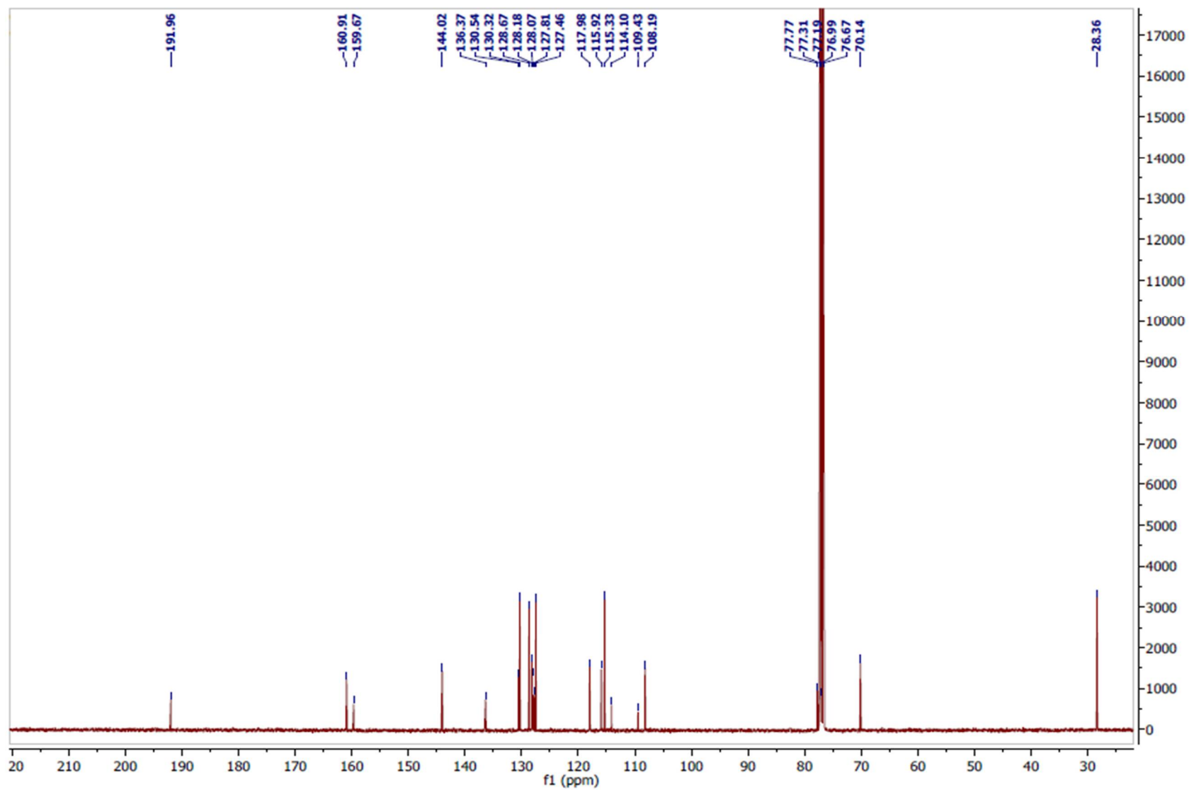
Page S6: Figure S4. 13 C NMR spectrum of 4-benzyloxylonchocarpin ( 1 ) (400 MHz, CDCl 3 ).
