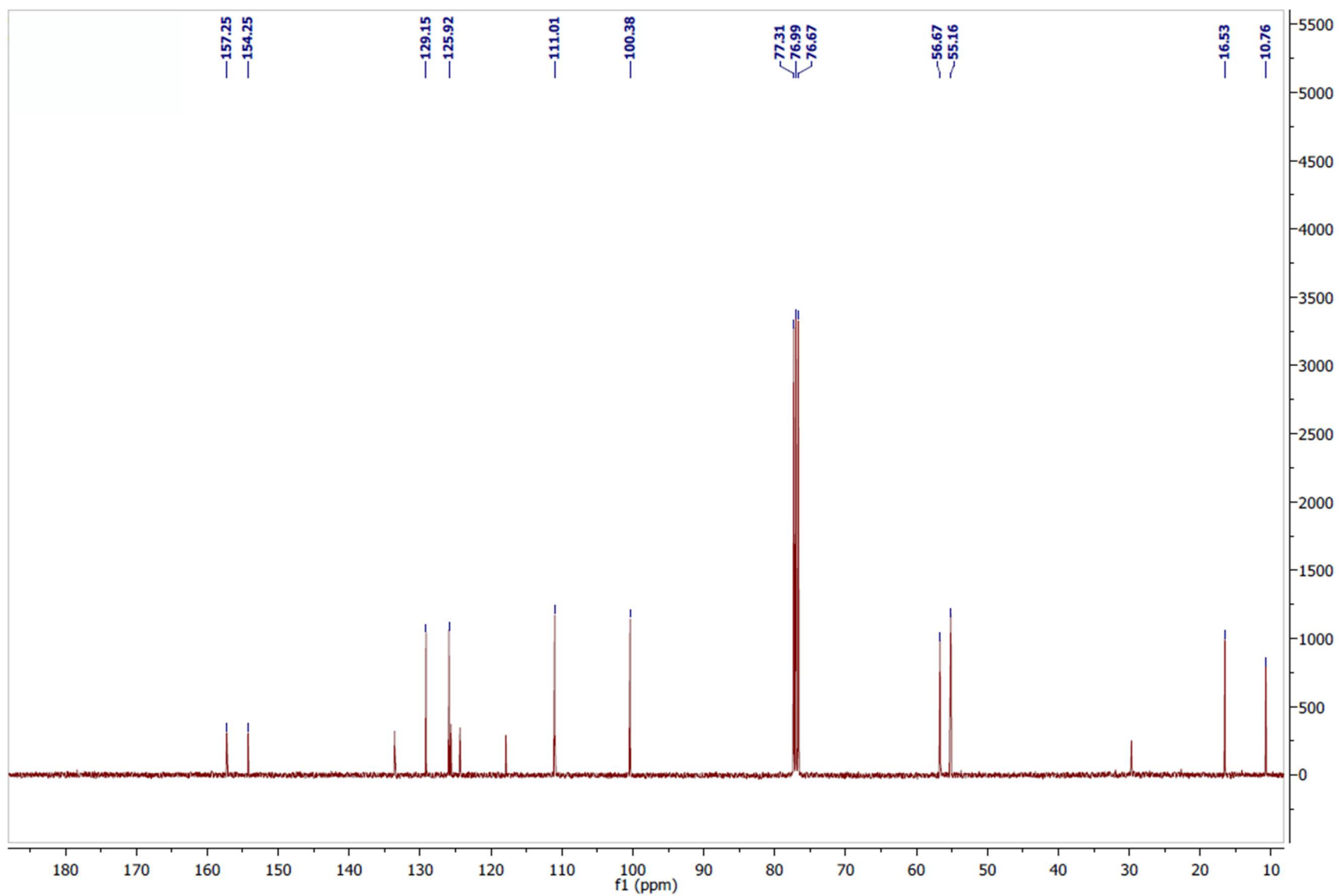
Page S25: Figure S23. ^{13}\text{C} NMR spectrum of muracatane C (4) (400 MHz, \text{CDCl}_3 ).
