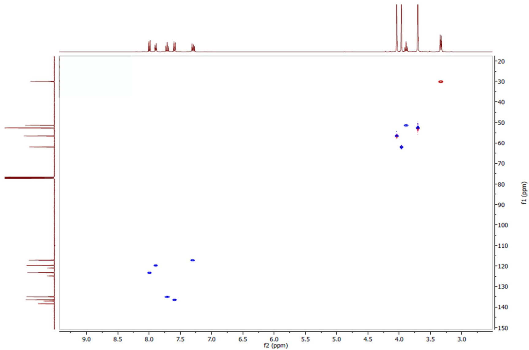
Page S15: Figure S13. HSQC spectrum of muracatane A (2) (400 MHz, CDCl 3 ).
