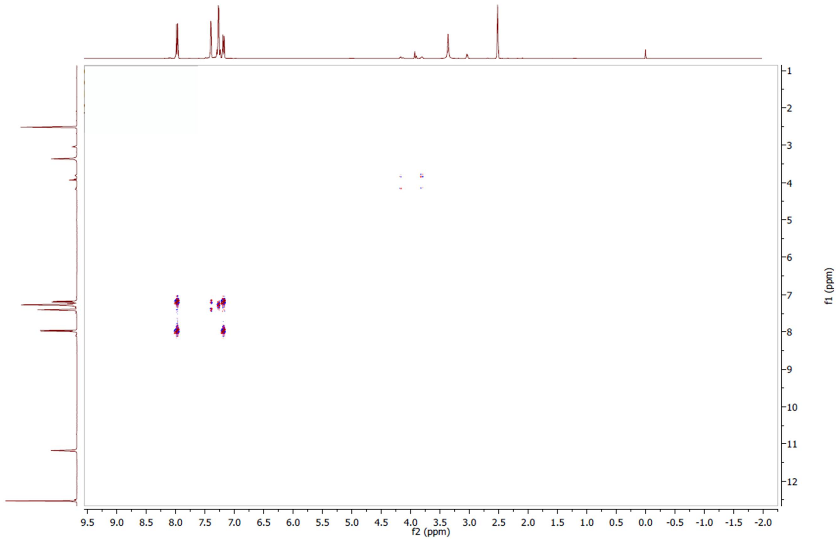
Page S20: Figure S18. COSY spectrum of muracatane B ( 3 ) (400 MHz, DMSO-d 6 ).
