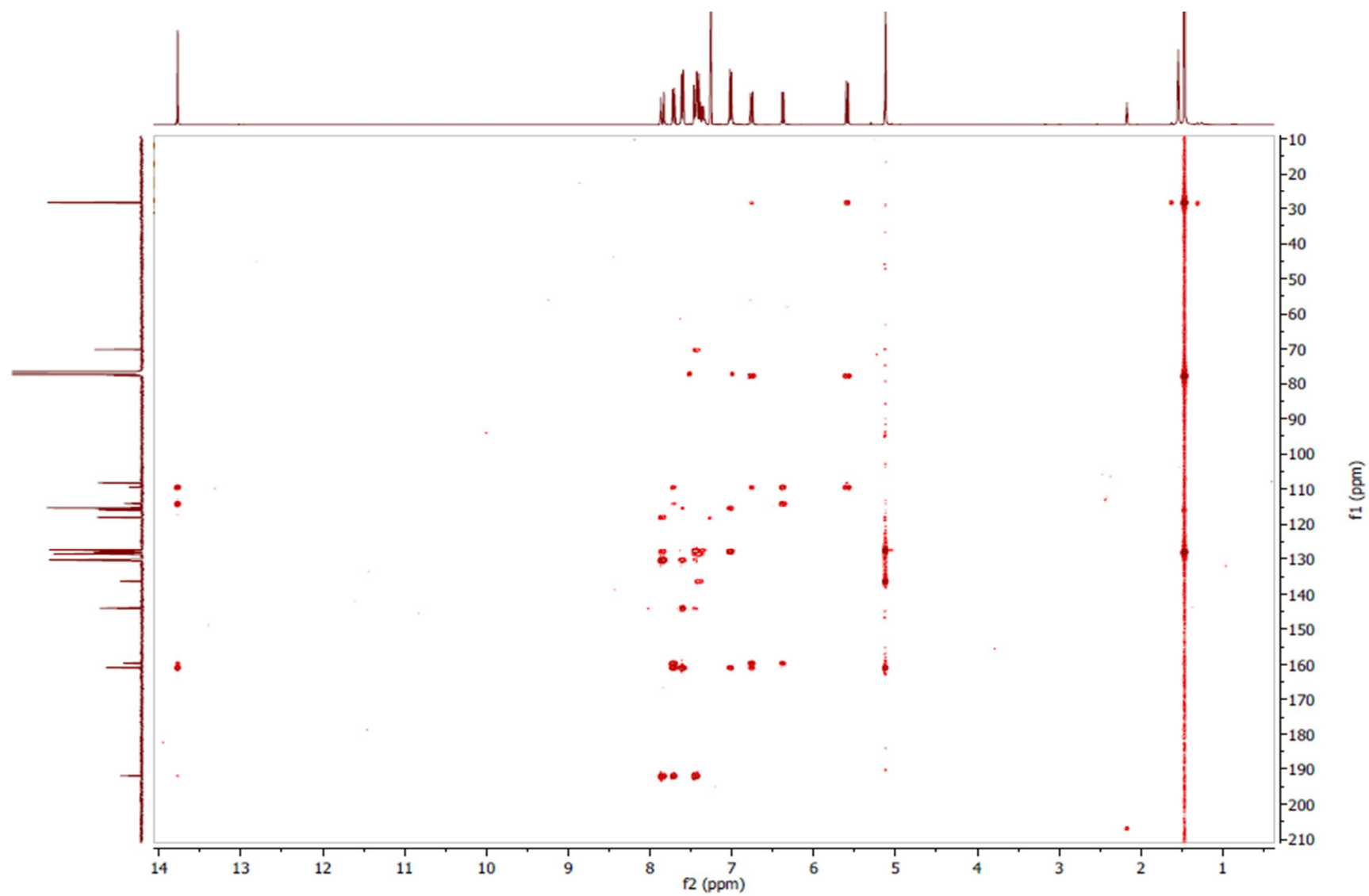
Page S9: Figure S7. HMBC spectrum of 4-benzyloxylonchocarpin ( 1 ) (400 MHz, CDCl 3 ).
