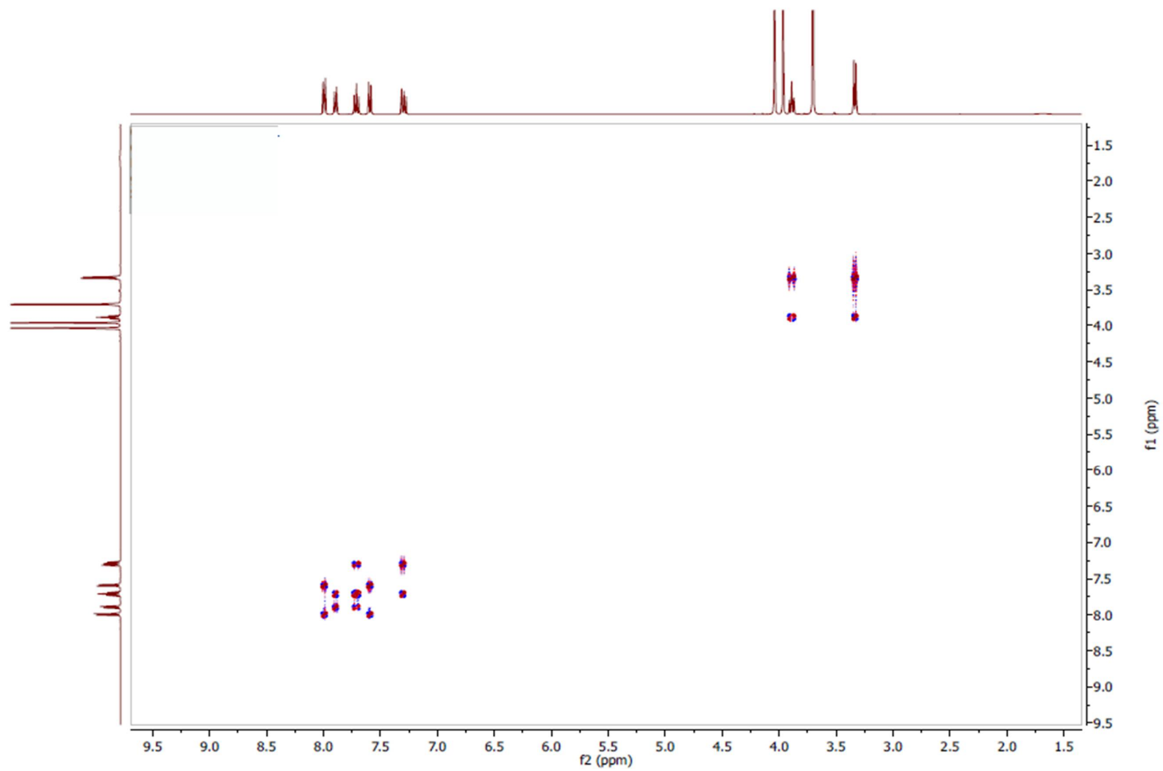
Page S14: Figure S12. COSY spectrum of muracatane A (2) (400 MHz, CDCl 3 ).
