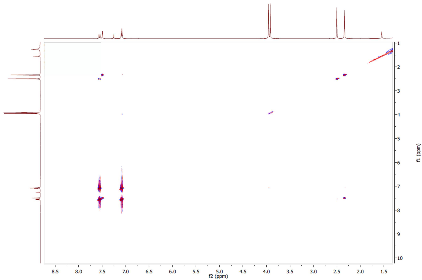
Page S27: Figure S25. COSY spectrum of muracatane C ( 4 ) (400 MHz, CDCl 3 ).
