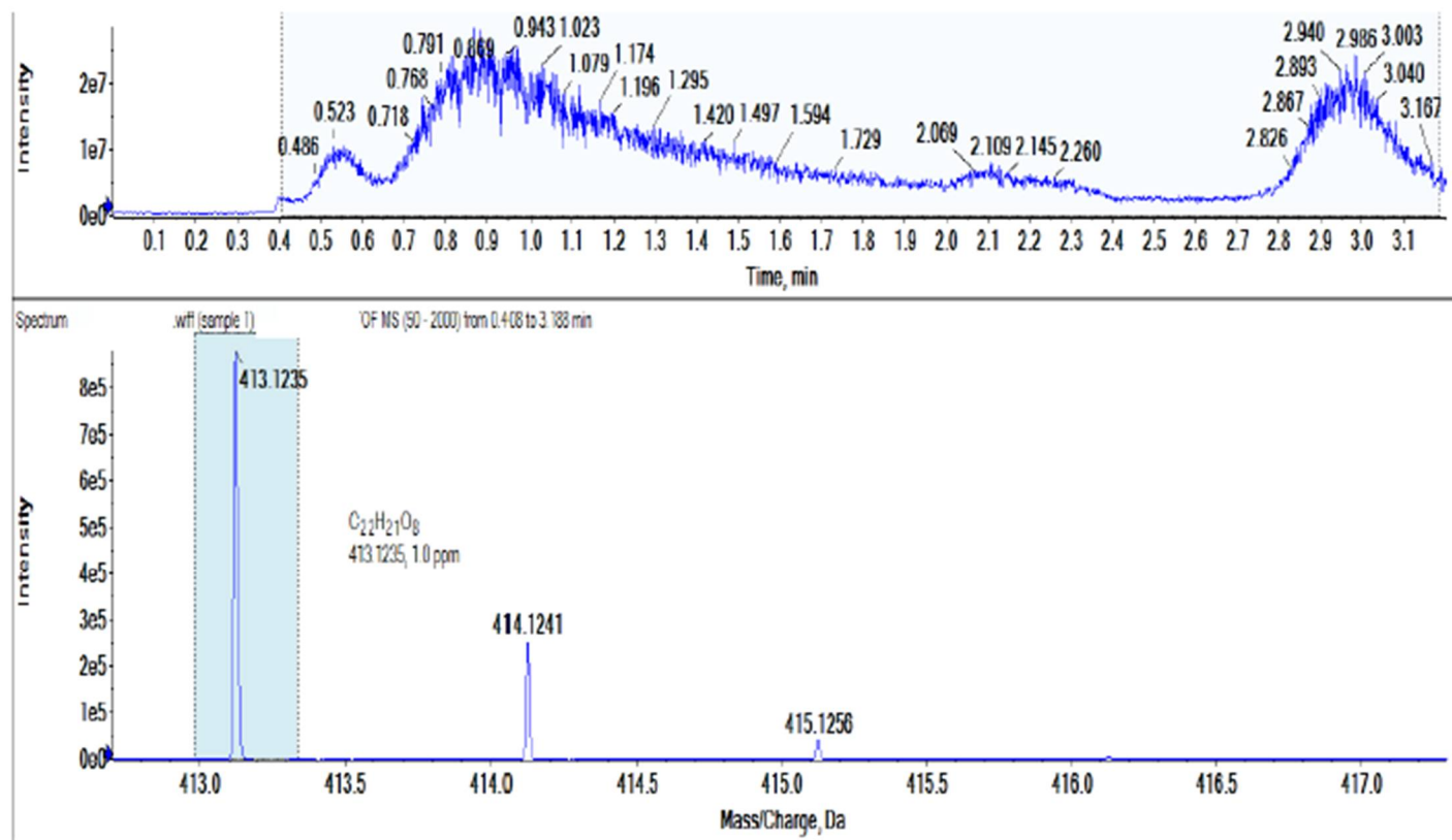
Page S17: Figure S15. HRESIMS spectrum of muracatane A (2).
