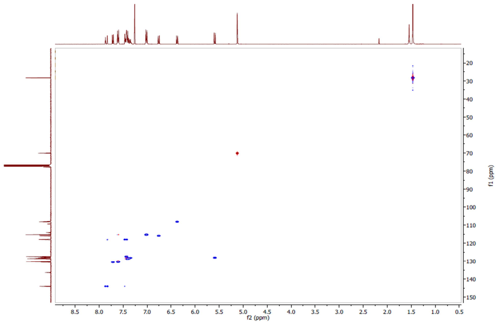
Page S8: Figure S6. HSQC spectrum of 4-benzyloxylonchocarpin ( 1 ) (400 MHz, CDCl 3 ).
