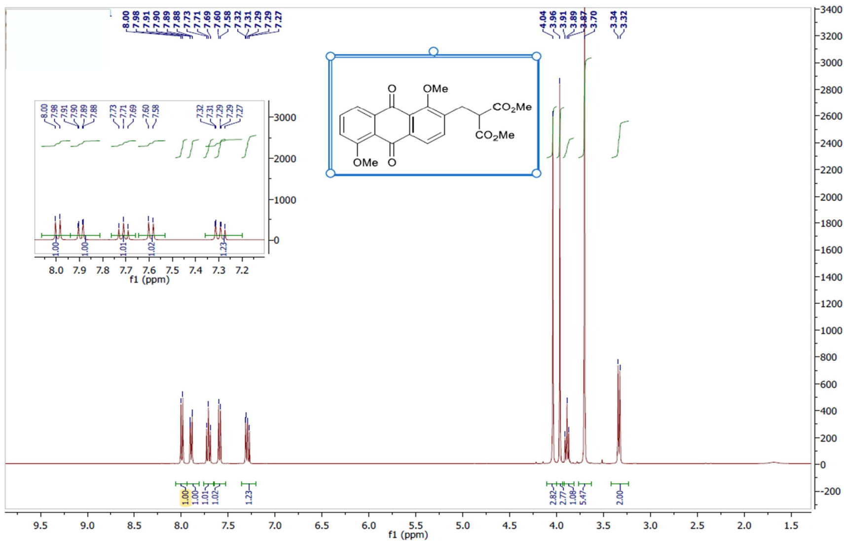
Page S11: Figure S9. ^1\text{H} NMR spectrum of muracatane A ( 2 ) (400 MHz, \text{CDCl}_3 ).
