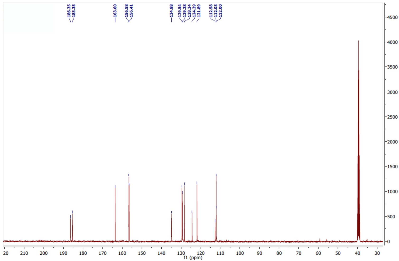
Page S19: Figure S17. 13 C NMR spectrum of muracatane B (3) (400 MHz, DMSO-d 6 ).
