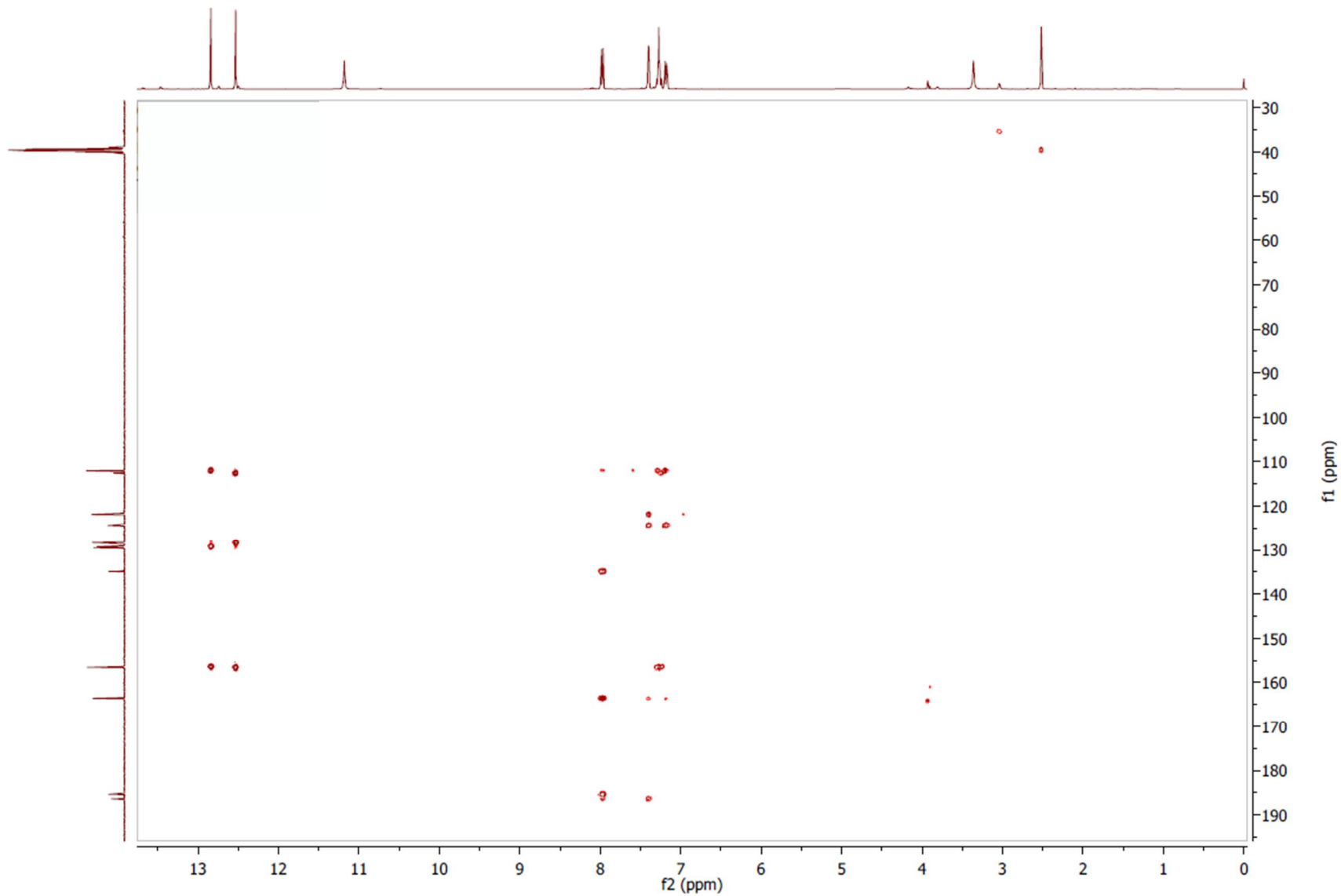
Page S22: Figure S20. HMBC spectrum of muracatane B (3) (400 MHz, DMSO-d 6 ).
