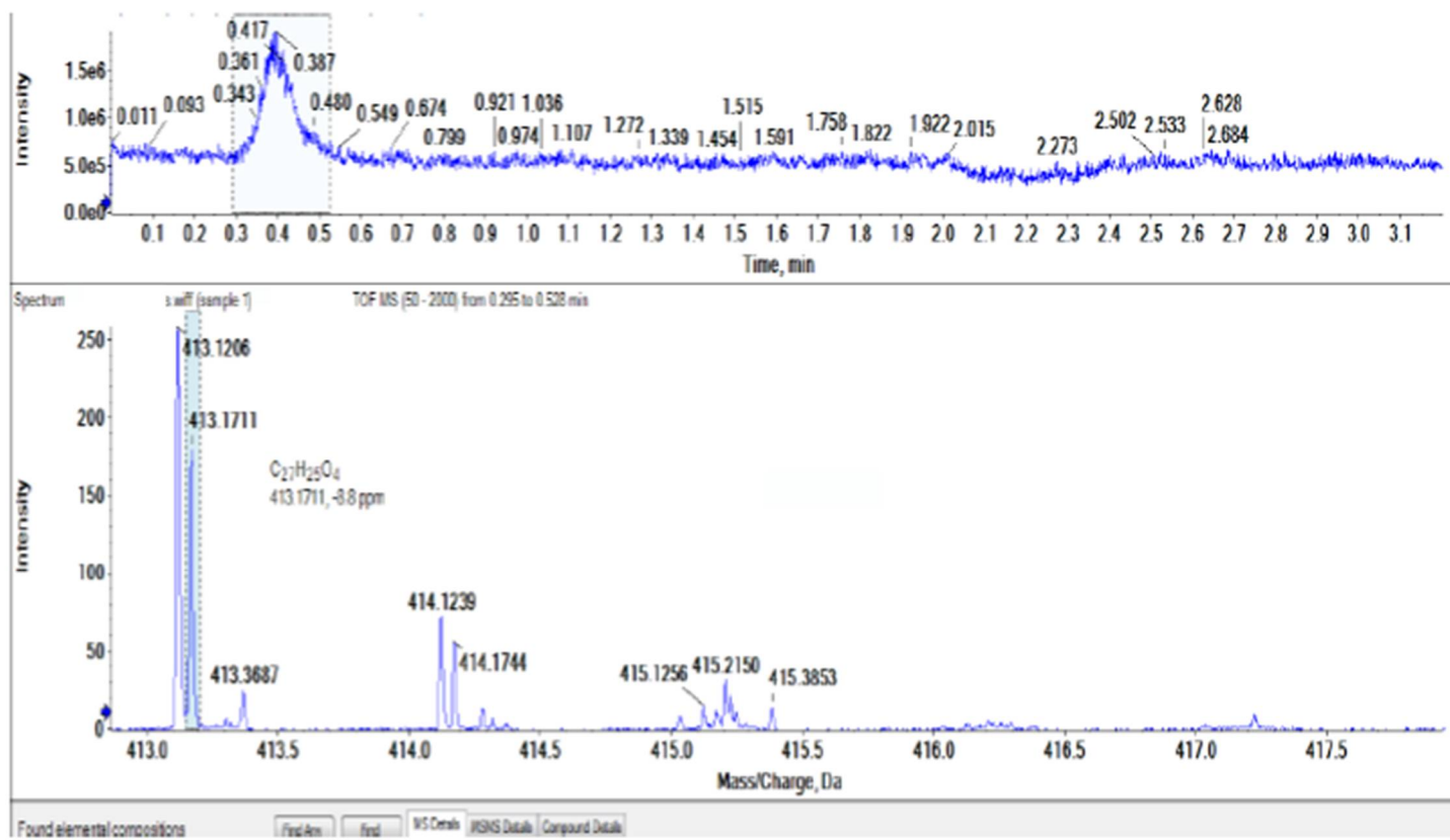
Page S10: Figure S8. HRESIMS spectrum of 4-benzyloxylonchocarpin ( 1 ).
