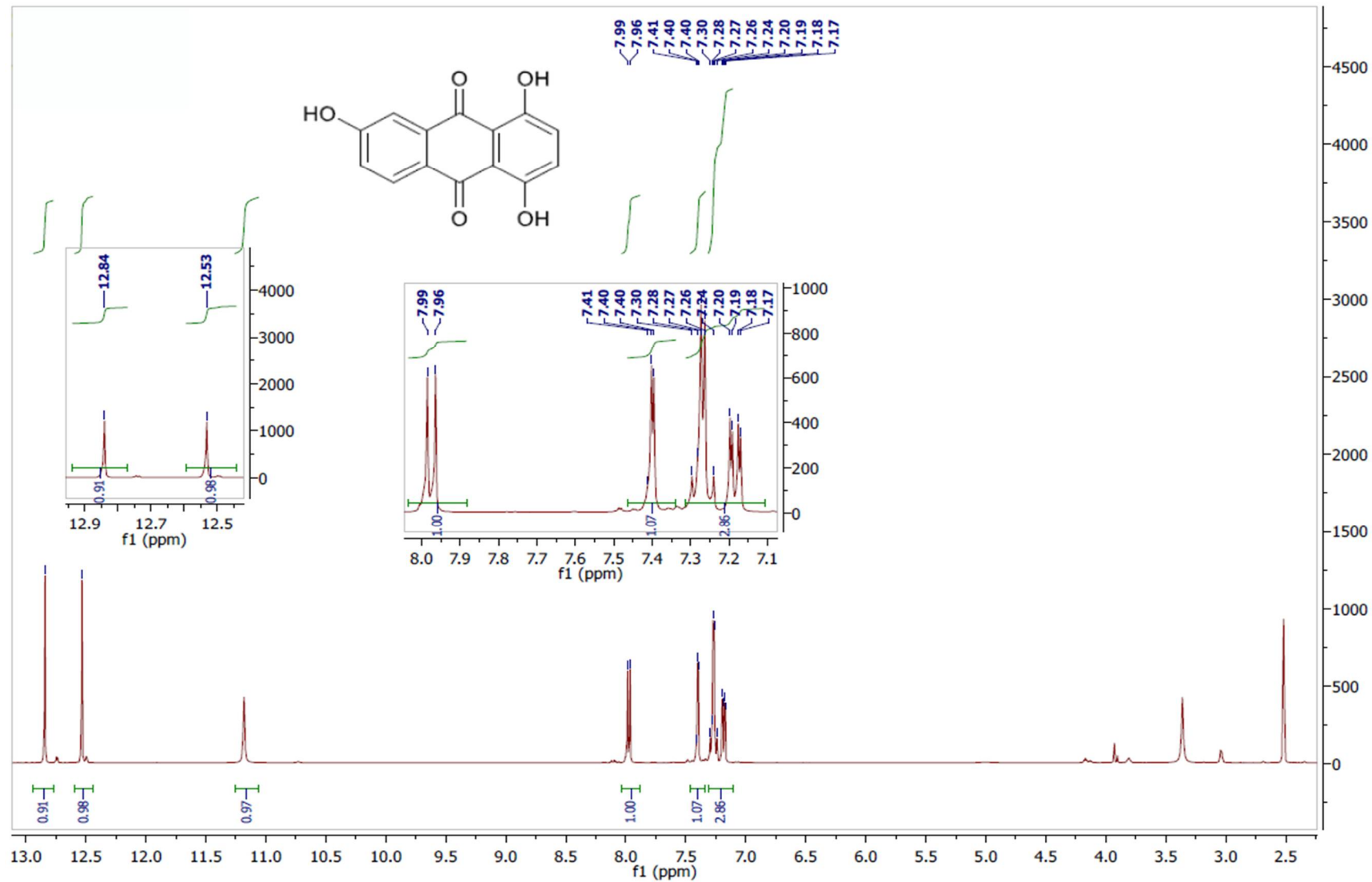
Page S18: Figure S16. 1 H NMR spectrum of muracatane B (3) (400 MHz, DMSO-d 6 ).
