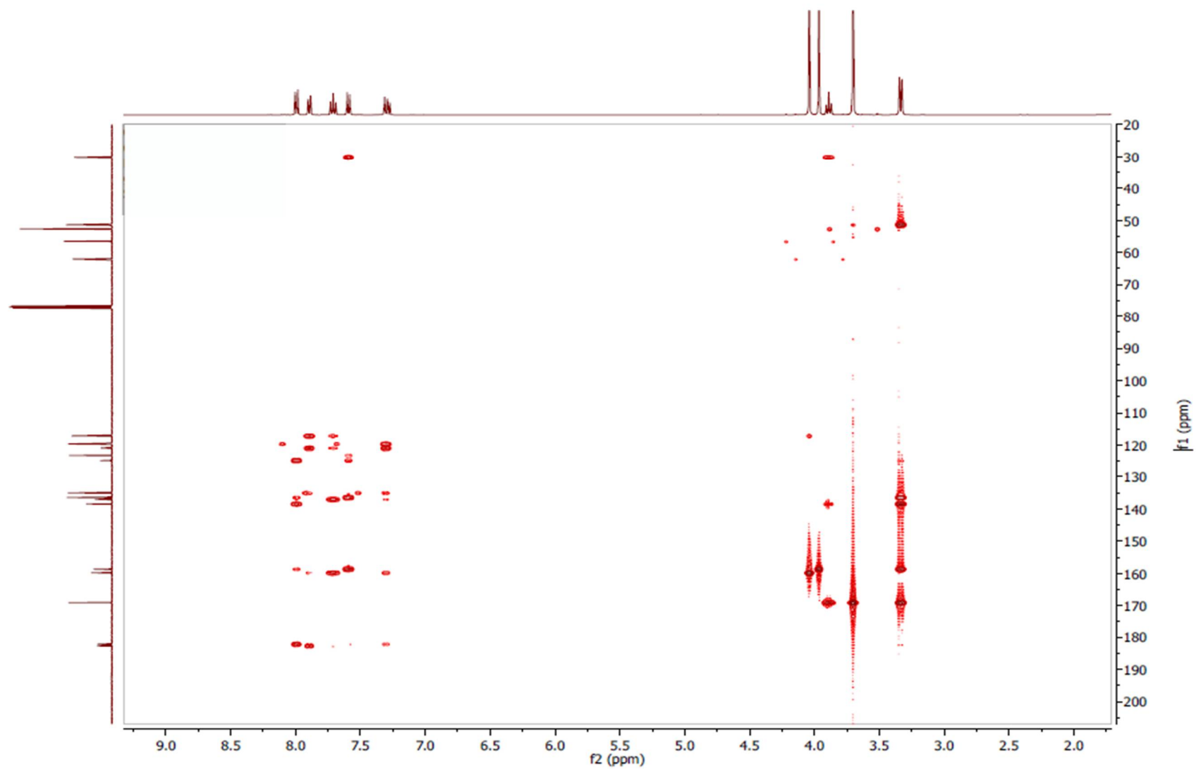
Page S16: Figure S14. HSQC spectrum of muracatane A (2) (400 MHz, CDCl 3 ).
