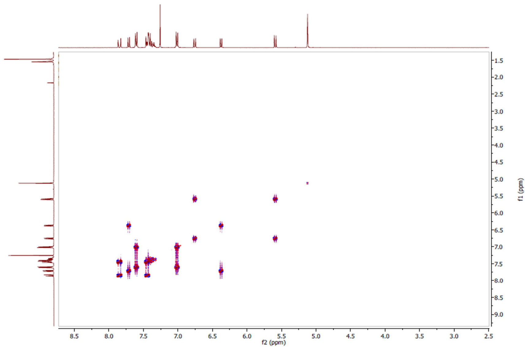
Page S7: Figure S5. COSY spectrum of 4-benzyloxylonchocarpin ( 1 ) (400 MHz, CDCl 3 ).
