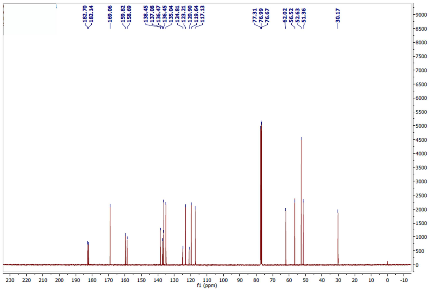
Page S12: Figure S10. ^{13}\text{C} NMR spectrum of muracatane A (2) (400 MHz, \text{CDCl}_3 ).
