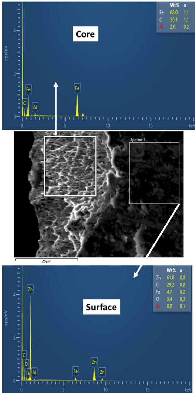
Figure S2. EDX of NW.
