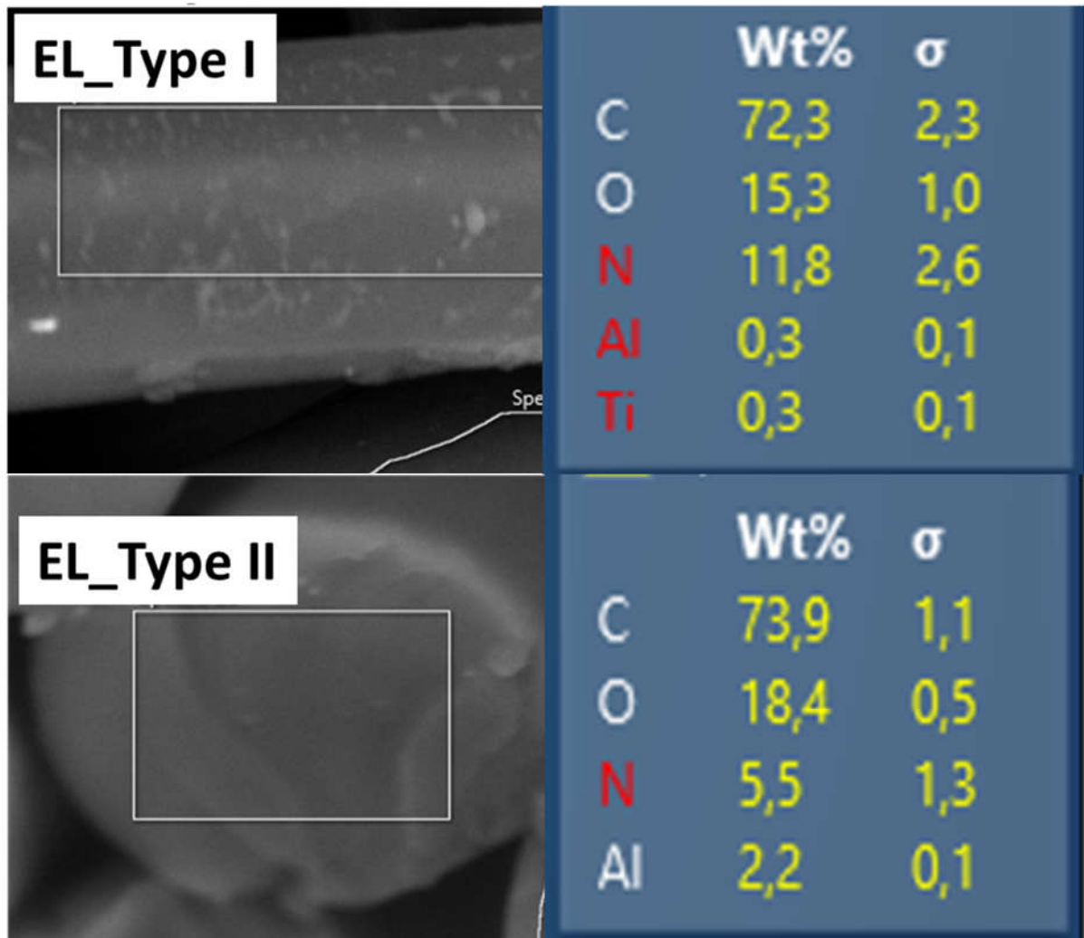
Figure S1. EDX of EL_Type I and EL_Type II.
