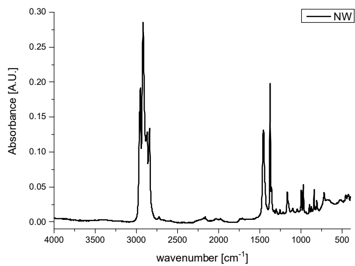
Figure S3. ATR of the surface of the NW.
