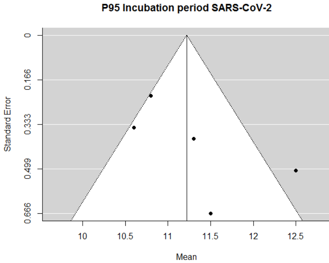
Figure S2. Funnel plot for assessing reporting bias for the 95%tile of the incubation period distribution
