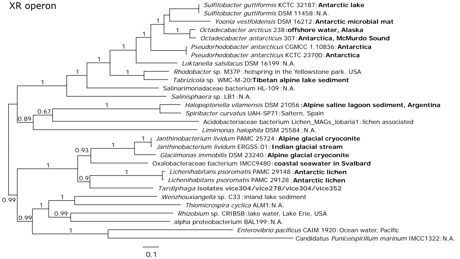
Figure S5 Maximum-likelihood phylogeny of the whole XR operon of Tardiphaga isolates and their top tBLASTn hits in NCBI's genome database.
