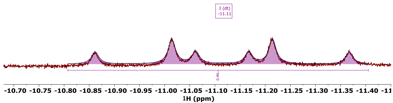
Figure S12. ^1\text{H} NMR spectrum of \{\text{MeP}_3\text{CoH}\}_2(\mu\text{-N}_2) at the hydride region with shading corresponding to the spin simulation.
