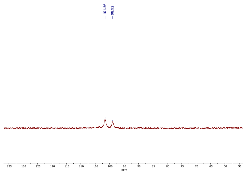
Figure S10. ^{31}\text{P} NMR spectrum of \{\text{Ph}^2\text{N}\text{P}_3\text{CoH}\}_2(\mu\text{-N}_2) .
