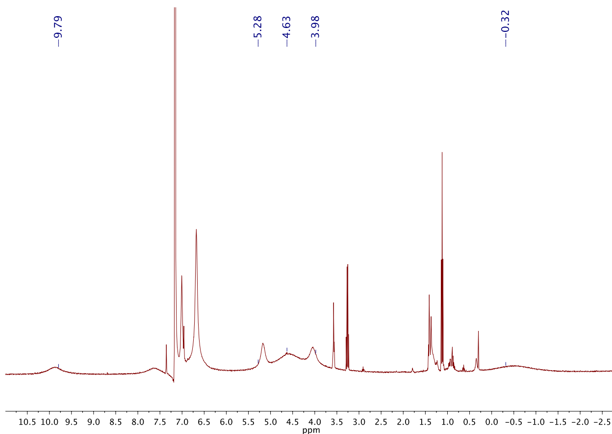
Figure S2. ^1\text{H NMR} spectrum of \text{Ph}_2\text{N-P}_3\text{CoCl}_2 .
