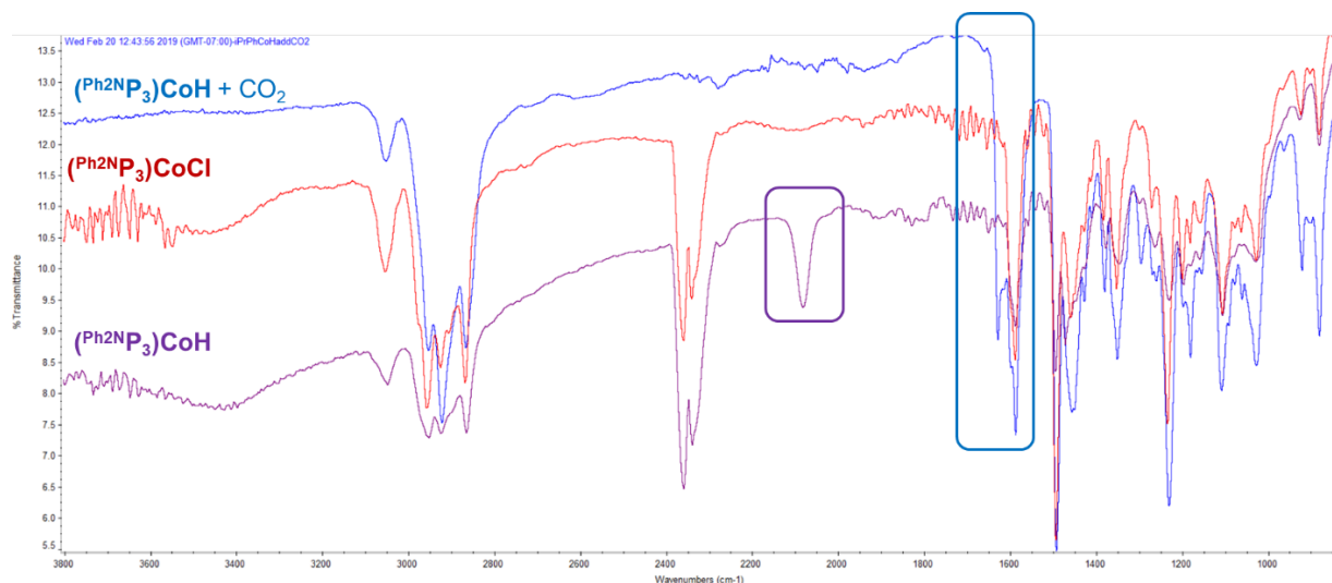
Figure S15. Stacked IR spectra for \text{Ph}^2\text{N}_3\text{CoX} . (purple): \text{Ph}^2\text{N}_3\text{CoH} , with the Co-H stretch shown in the purple box at 2082\text{ cm}^{-1} . (red): \text{Ph}^2\text{N}_3\text{CoCl} . (blue): \text{Ph}^2\text{N}_3\text{CoH} + \text{CO}_2 . A new stretch at 1628\text{ cm}^{-1} is indicative of formation of a formate species such as \text{Ph}^2\text{N}_3\text{Co-OCHO} .
