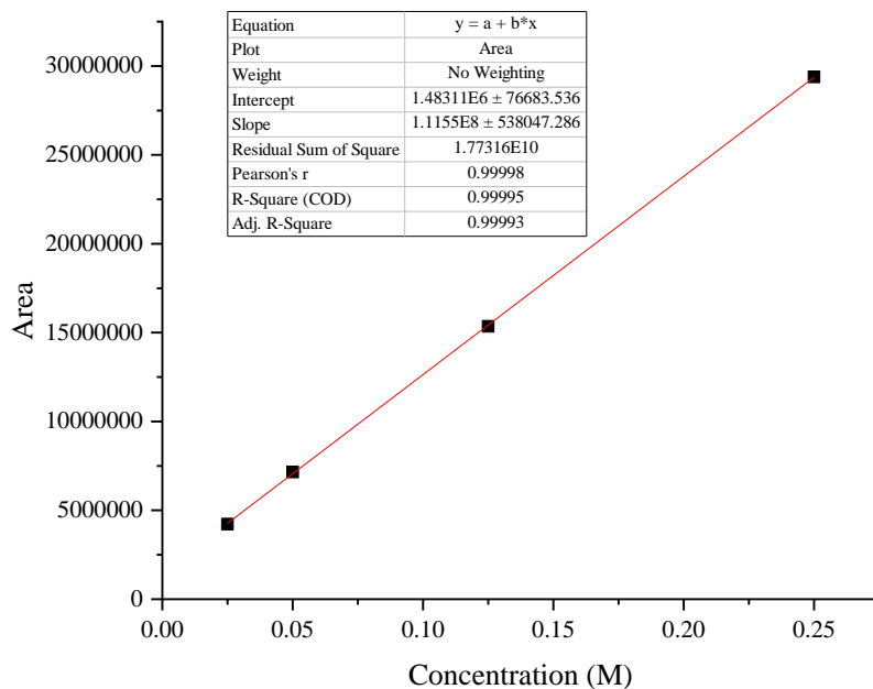
Figure S22. Calibration curve for MeOH detection.
