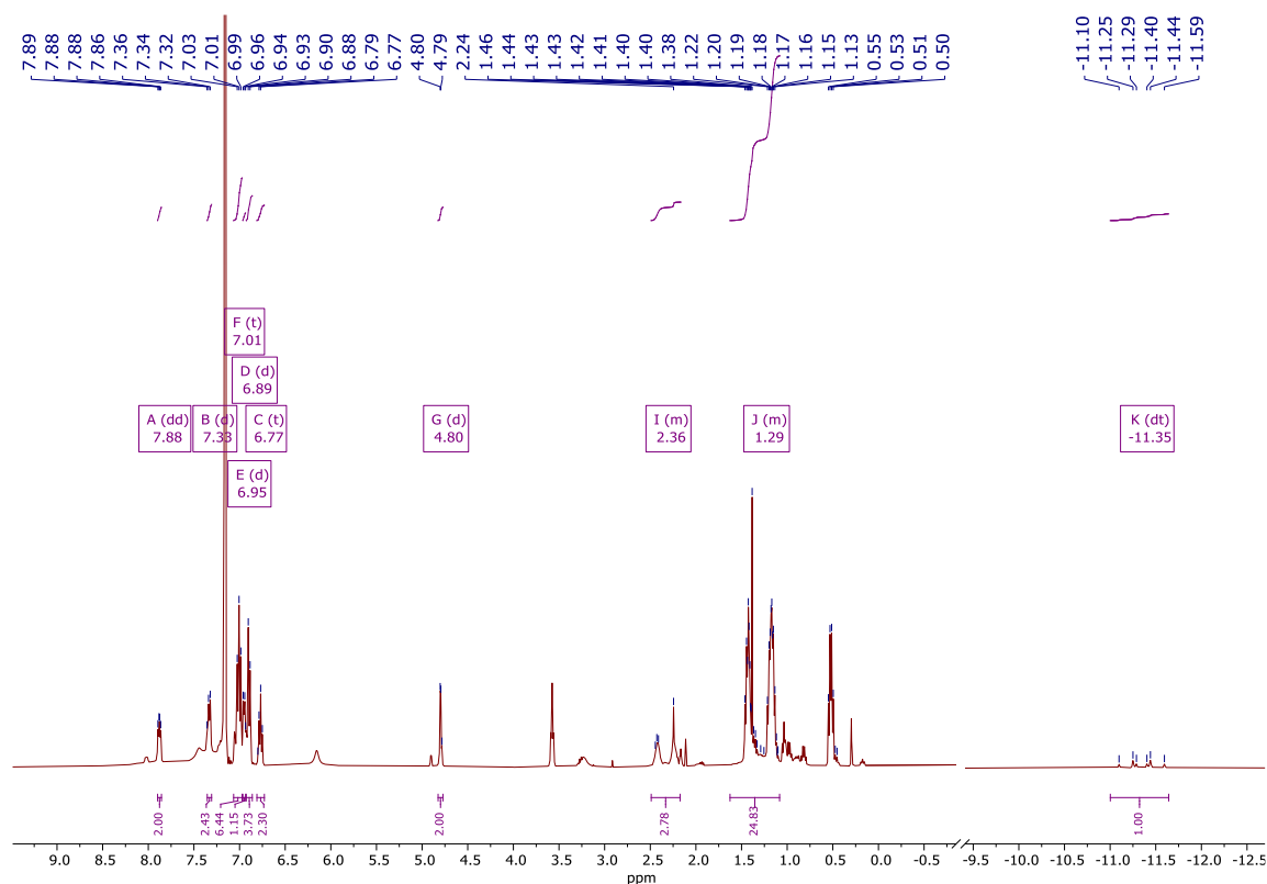
Figure S7. ^1\text{H} NMR spectrum of \{\text{Ph}_2\text{N-P}_3\text{CoH}\}_2(\mu\text{-N}_2) .
