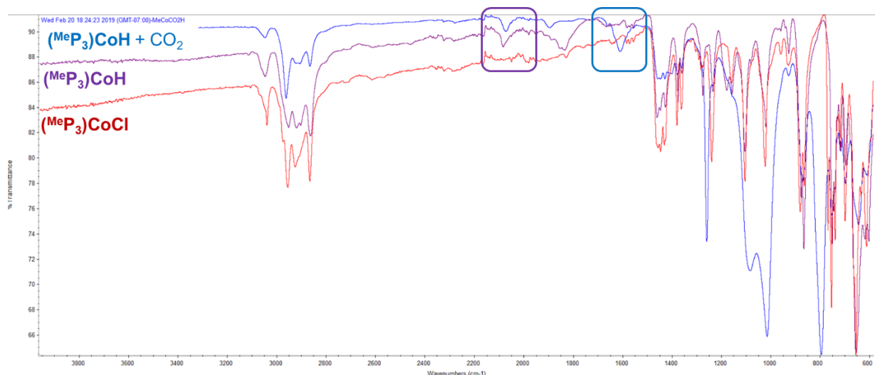
Figure S16. Stacked IR spectra for \text{Me}^3\text{P}_3\text{CoX} . (purple): \text{Me}^3\text{P}_3\text{CoH} , with the Co-H stretch shown in the purple box at 2084\text{ cm}^{-1} . (red): \text{Me}^3\text{P}_3\text{CoCl} . (blue): \text{Me}^3\text{P}_3\text{CoH} + \text{CO}_2 . A new stretch at 1610\text{ cm}^{-1} is indicative of formation of a formate species such as \text{Me}^3\text{P}_3\text{Co-OCHO} . The presence of a hydride resonance in this spectrum is consistent with the NMR data.
