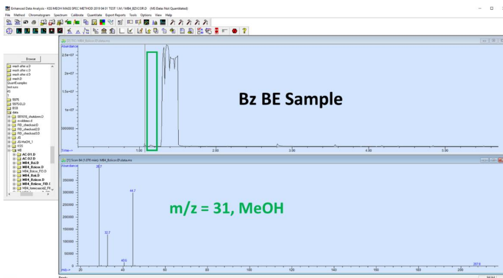
Figure S23. GC (top) and MS (bottom) of the vac-transferred liquid phase after bulk electrolysis with (^{Bz2N}P_3)CoCl . The green boxed area shows MeOH (and MeCN) by GC. Spiking the solution with MeOH showed an increase in the boxed area. The other areas correspond to MeCN.
