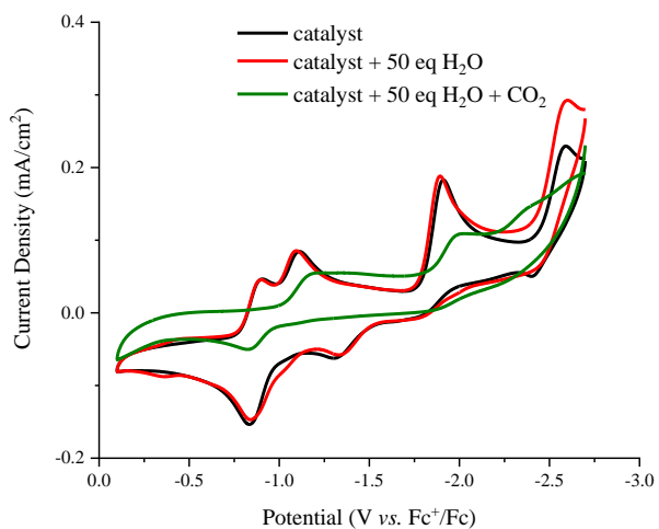
Figure S30. Cyclic voltammograms of 1 mM [\text{Ph}_2\text{N}]\text{P}_3\text{Co}(\text{MeCN})[\text{BARF}] under various conditions; under \text{N}_2 (black), in the presence of 50 eq \text{H}_2\text{O} (red), and in the presence of 50 eq \text{H}_2\text{O} and \text{CO}_2 (green). Conditions: GC working electrode, 0.1 M \text{TBAPF}_6/\text{MeCN} solvent, scan rate of 0.06 V/s, scanning negative, sweep 2 and 3, within -2.7 and 0 V vs. \text{Fc}^+/\text{Fc} .
