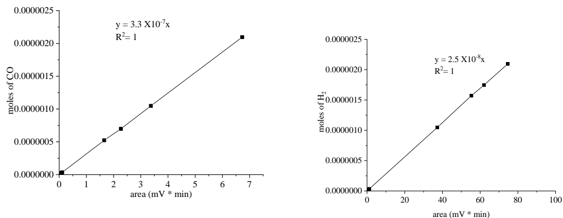
Figure S21. Calibration curve for CO (left) and H 2 (right) gas.
