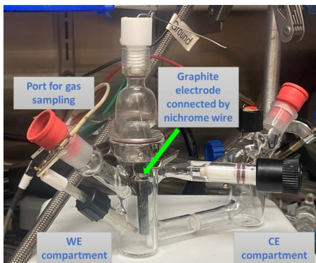
Figure S20. Typical H-cell set-up for BE in the glovebox.
