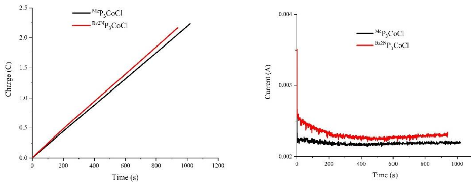
Figure S37. Charge vs. time ( left ) and current vs. time ( right ) for controlled potential electrolysis of the catalysts at -2.1 V vs. \text{Fc}^{+/0} .
