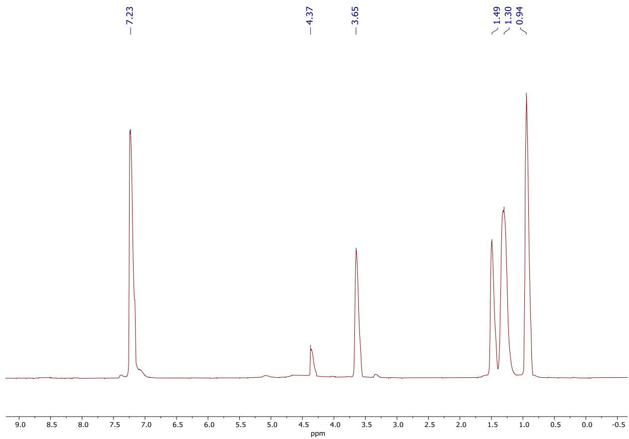
Figure S1. ^1\text{H} NMR spectrum of \text{Bz}_2\text{NP}_3\text{CoCl}_2 .
