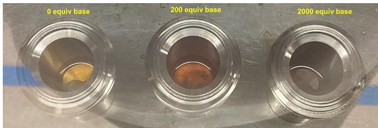
Figure S18. Photograph showing the discoloration of \text{Bz}_2\text{N-P}_3\text{CoCl} upon addition of base.
