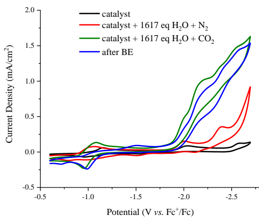
Figure S33. Cyclic voltammograms of 1 mM \text{MeP}_3\text{CoCl} under various conditions during BE; under \text{N}_2 (black), in the presence of 1617 eq (3%) \text{H}_2\text{O} (red), in the presence of 1617 eq (3%) \text{H}_2\text{O} and \text{CO}_2 (green), and after 15 min of BE (blue). Conditions: GC working electrode, 0.1 M \text{TBAPF}_6/\text{MeCN} solvent, scan rate of 0.1 V/s, scanning negative, within 0 and -2.7 V vs. \text{Fc}^+/\text{Fc} .
