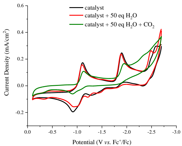
Figure S27. Cyclic voltammograms of 1 mM \text{Ph}_2\text{N-P}_3\text{CoCl} under various conditions; under \text{N}_2 (black), in the presence of 50 eq \text{H}_2\text{O} (red), and in the presence of 50 eq \text{H}_2\text{O} and \text{CO}_2 (green). Conditions: GC working electrode, 0.1 M \text{TBAPF}_6/\text{MeCN} solvent, scan rate of 0.06 V/s, scanning negative, sweep 2 and 3, within -2.7 and 0 V vs. \text{Fc}^+/\text{Fc} .
