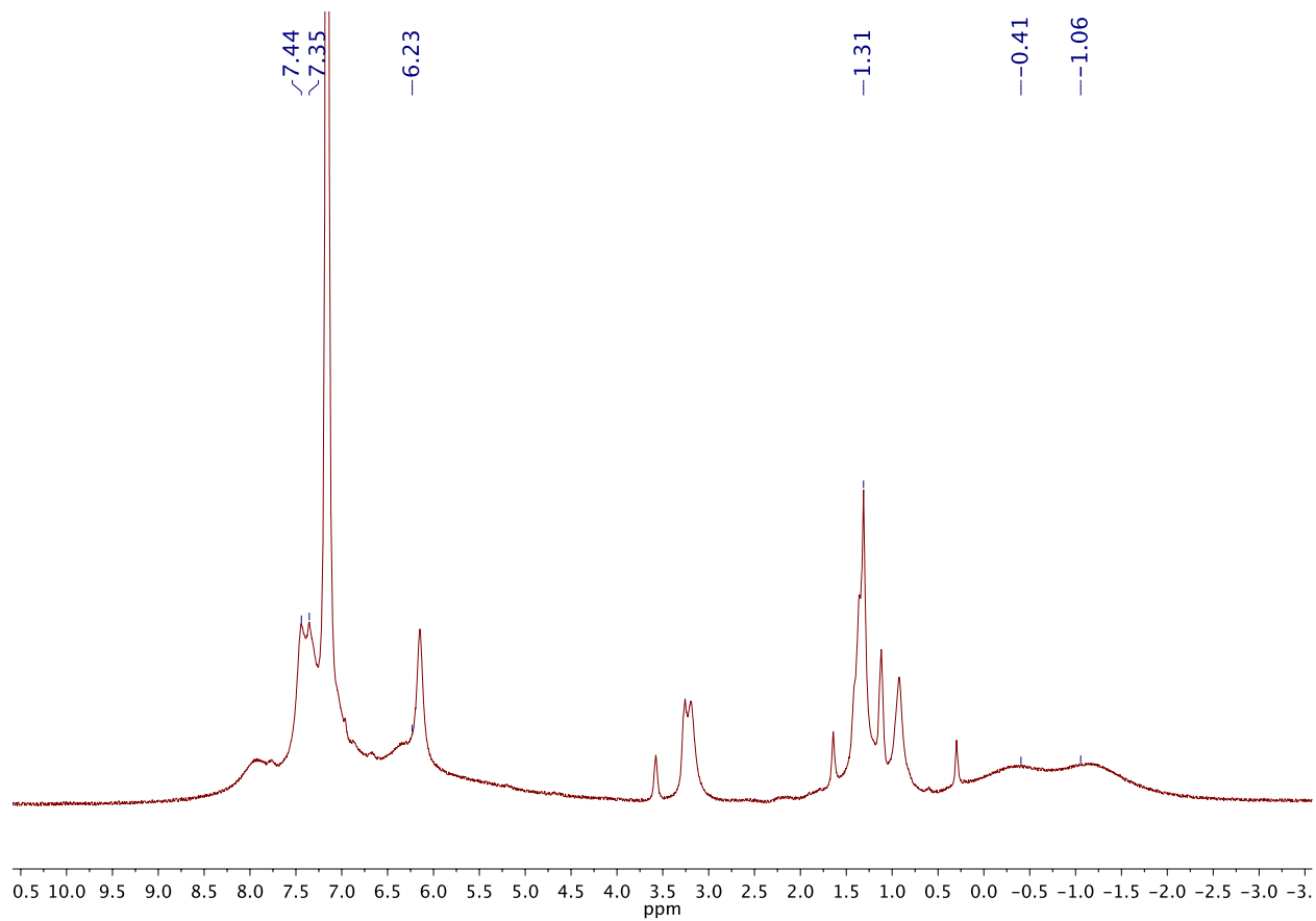
Figure S5. ^1\text{H} NMR spectrum of \text{Ph}_2\text{N-P}_3\text{CoCl} .
