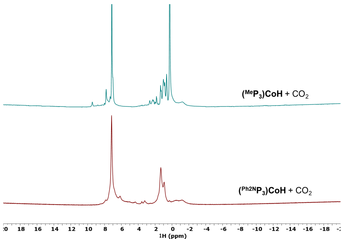
Figure S14. ^1\text{H} NMR spectra ( \text{C}_6\text{D}_6 ) of the reactions of the Co-H species with \text{CO}_2 , taken at t = 3 hours.
