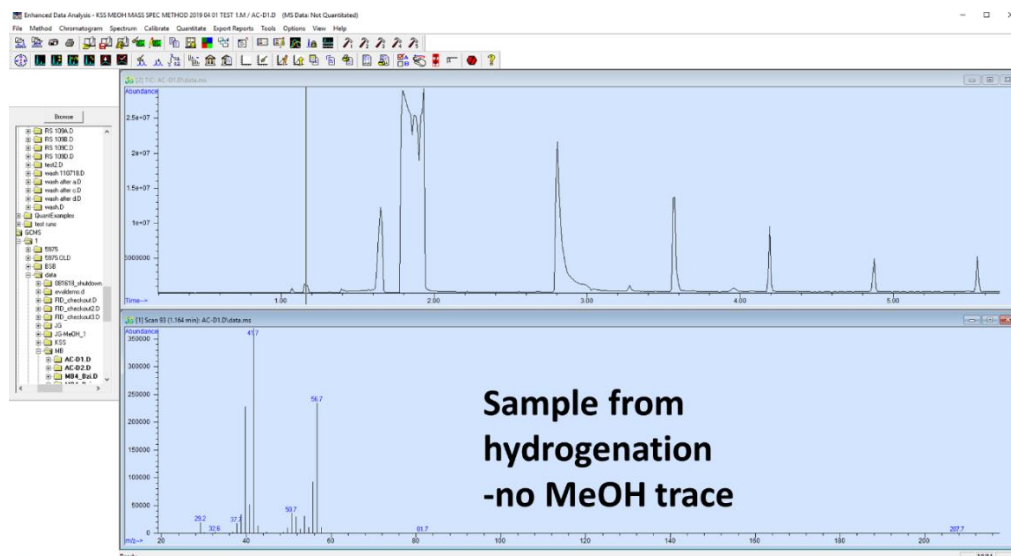
Figure S24. GC (top) and MS (bottom) of the solution after hydrogenation with (^{Bz_2N}P_3)CoCl . No MeOH is present.
