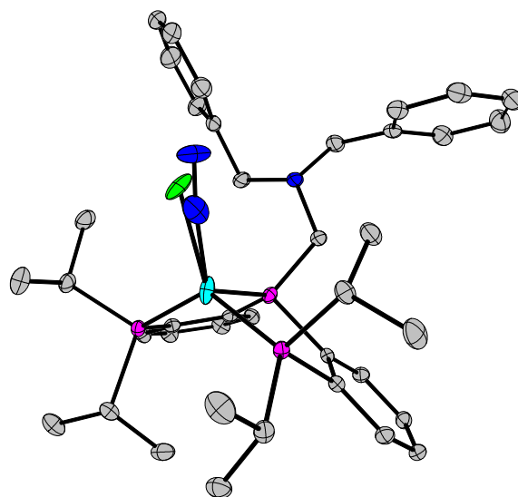
Figure S17. Thermal ellipsoid plot of Bz_2N_3P_3Co(N_2) . The crystal contains 33% impurity of the starting Co(I)Cl. H-atoms omitted for clarity.
