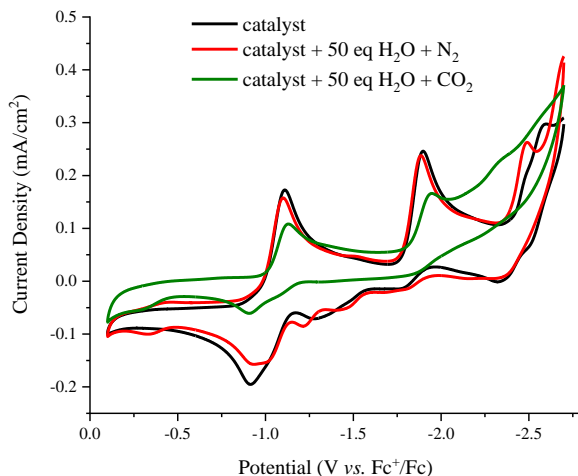
Figure S32. Cyclic voltammograms of 1 mM \text{MeP}_3\text{CoCl} under various conditions; under \text{N}_2 (black), in the presence of 50 eq \text{H}_2\text{O} (red), and in the presence of 50 eq of \text{H}_2\text{O} and \text{CO}_2 (green). Conditions: GC working electrode, 0.1 M \text{TBAPF}_6/\text{MeCN} solvent, scan rate of 0.06 V/s, scanning negative, sweep 2 and 3, within -2.7 and 0 V vs. \text{Fc}^+/\text{Fc} .
