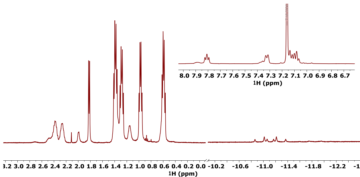
Figure S11. ^1\text{H} NMR spectrum of \{\text{MeP}_3\text{CoH}\}_2(\mu\text{-N}_2) . Inset shows the aromatic regions.
