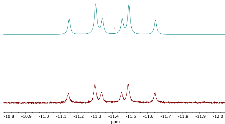
Figure S8. Hydride region of the ^1\text{H} NMR spectrum of \{\text{Ph}^{2\text{N}}\text{P}_3\text{CoH}\}_2 ( \mu\text{-N}_2 ). ( top ): Simulated by MestReNova using the coupling indicated above and ( bottom ): experimental.
