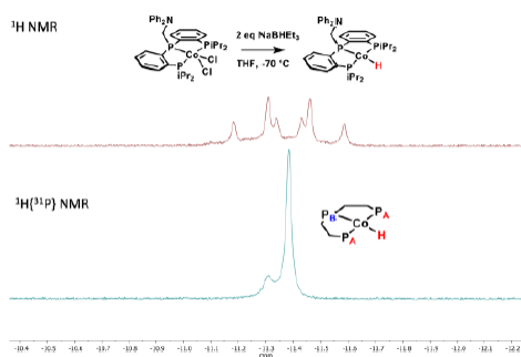
Figure S9. Hydride region of the ^1\text{H} (top) and ^1\text{H}\{^{31}\text{P}\} NMR spectrum of \{\text{Ph}^{2\text{N}}\text{P}_3\text{CoH}\}_2 ( \mu\text{-N}_2 ), showing the presence of a second hydride species. The two hydride resonances are speculated to correspond to the monomer (as drawn) and the \text{N}_2 -bridged dimer (as present in the solid-state).
