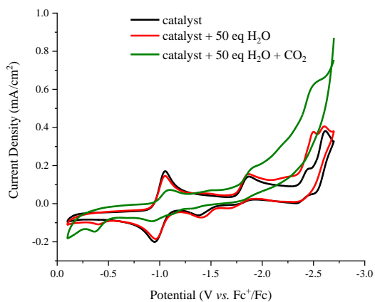
Figure S35. Cyclic voltammograms of 1 mM \text{Bz}_2\text{N-P}_3\text{CoCl} under various conditions; under \text{N}_2 (black), in the presence of 50 eq \text{H}_2\text{O} (red), and in the presence of 50 eq of \text{H}_2\text{O} and \text{CO}_2 (green). Conditions: GC working electrode, 0.1 M \text{TBAPF}_6/\text{MeCN} solvent, scan rate of 0.06 V/s, scanning negative, sweep 2 and 3, within -2.7 and 0 V vs. \text{Fc}^+/\text{Fc} .
