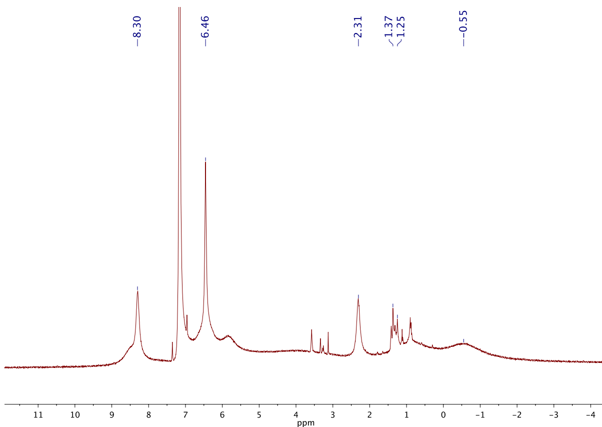
Figure S4. ^1\text{H} NMR spectrum of \text{Bz}_2\text{N-P}_3\text{CoCl} .
