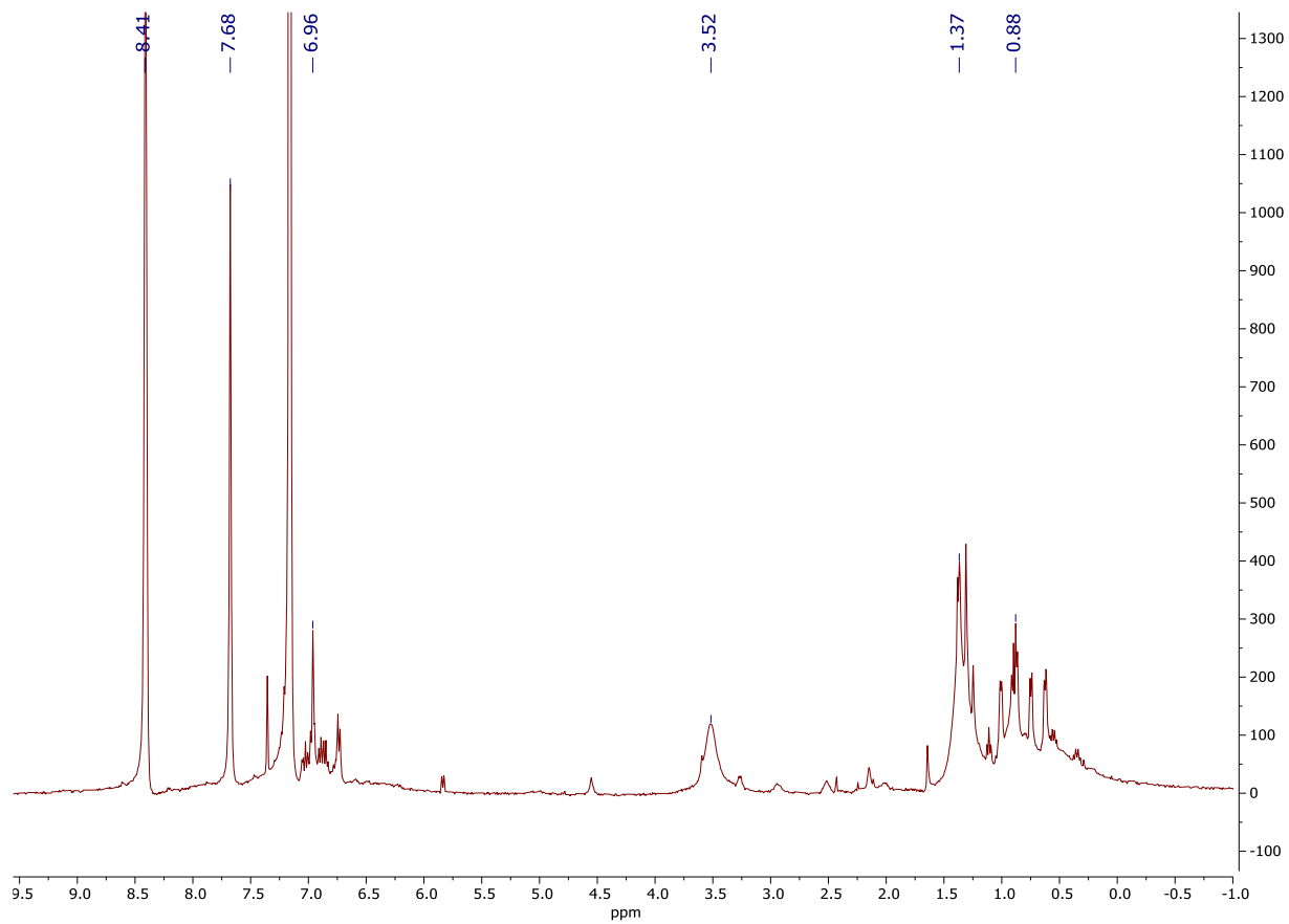
Figure S6. ^1\text{H} NMR spectrum of [\text{Ph}_2\text{N}]\text{P}_3\text{Co}(\text{MeCN})[\text{BArF}] .
