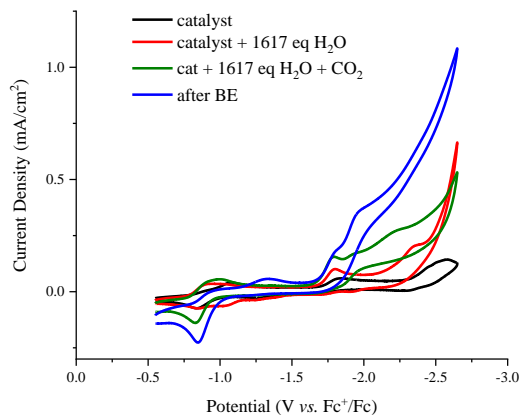
Figure S36. Cyclic voltammograms of 1 mM \text{Bz}_2\text{Np}_3\text{CoCl} under various conditions during BE; under \text{N}_2 (black), in the presence of 1617 eq (3%) \text{H}_2\text{O} (red), in the presence of 1617 eq (3%) \text{H}_2\text{O} and \text{CO}_2 (green), and after 15 min of BE (blue). Conditions: GC working electrode, 0.1 M \text{TBAPF}_6/\text{MeCN} solvent, scan rate of 0.1 V/s, scanning negative, within 0 and -2.7 V vs. \text{Fc}^+/\text{Fc} .
