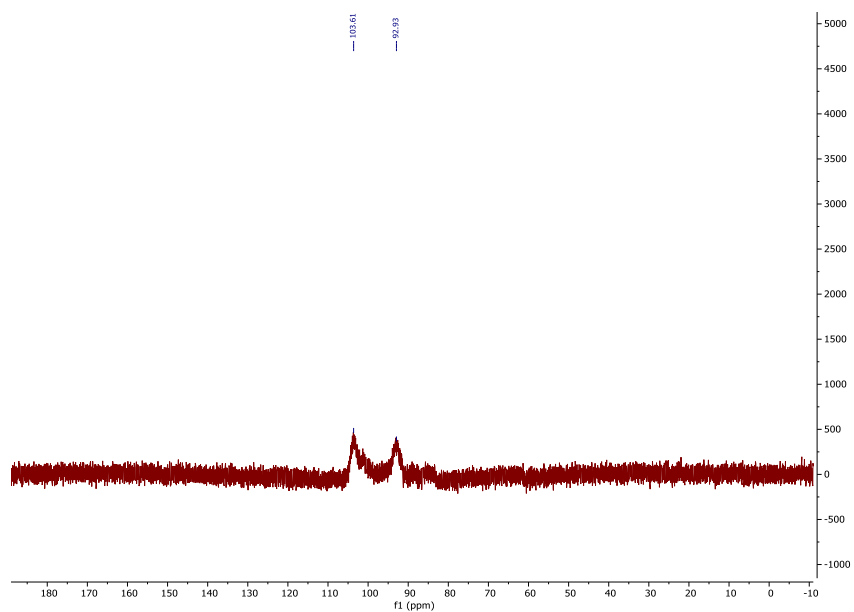
Figure S13. ^{31}\text{P} NMR spectrum of \{\text{MeP}_3\text{CoH}\}_2(\mu\text{-N}_2) .
