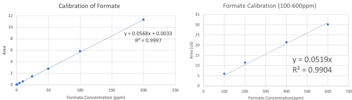
Figure S19. Calibration curves for formate detection, spanning two different ranges.
