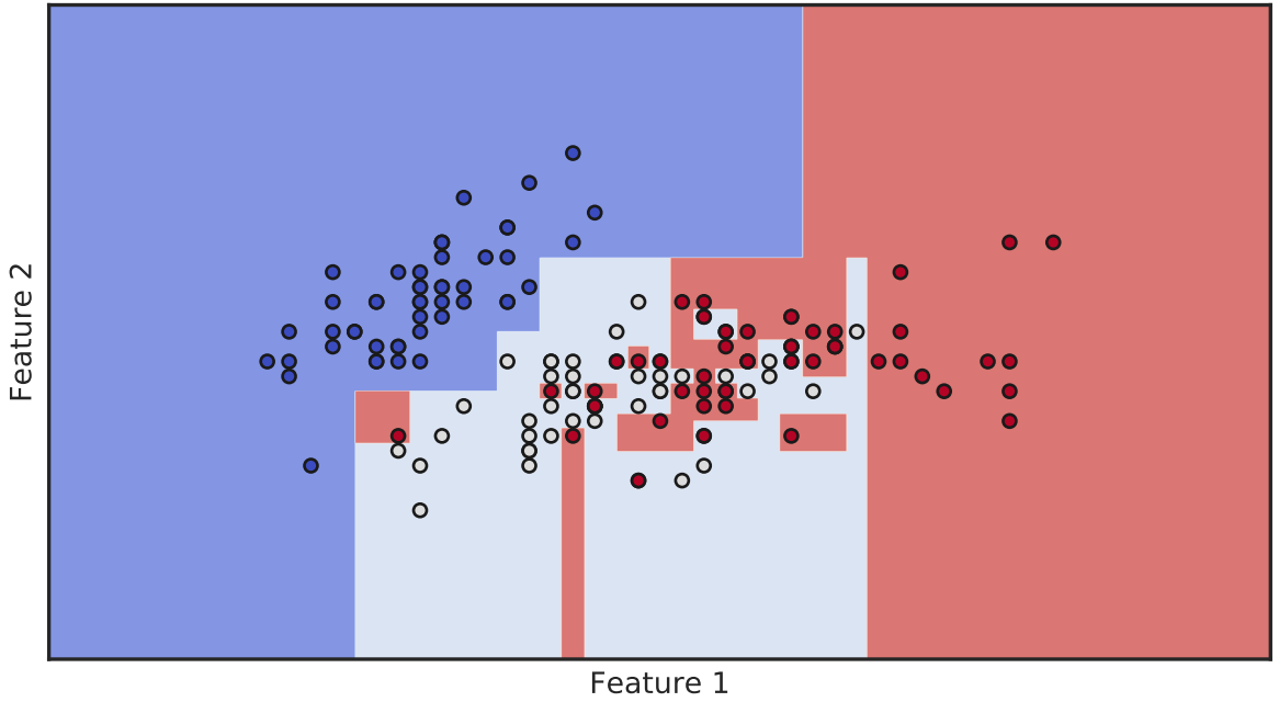
Decision tree
