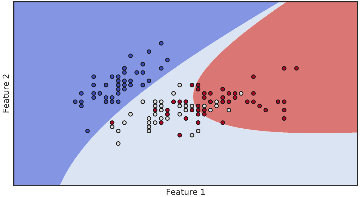
SVM with nonlinear kernel
