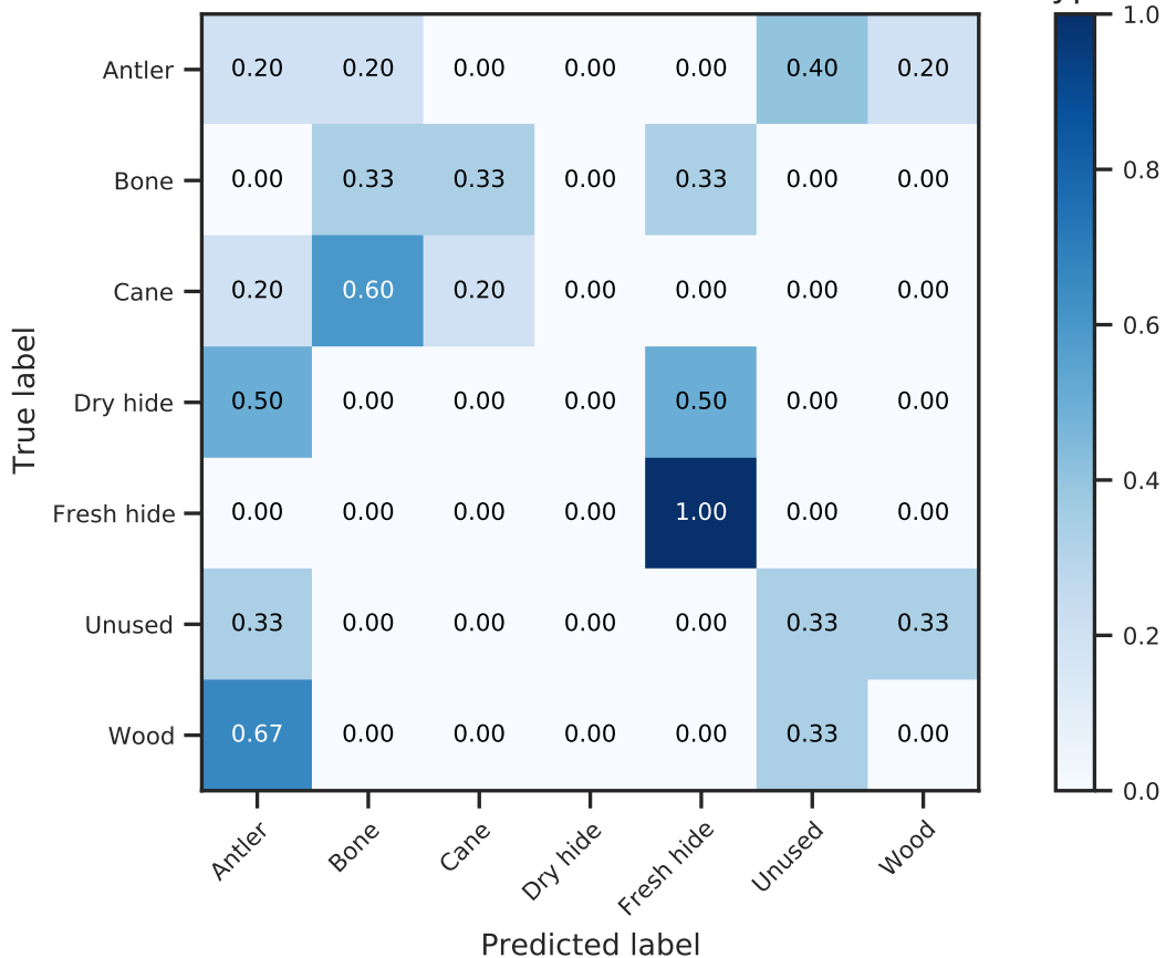
Normalized confusion matrix on test for SVM2 without type
