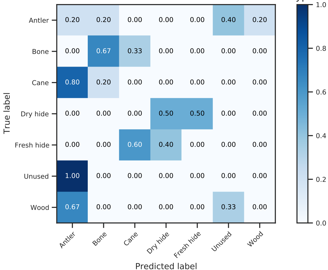
Normalized confusion matrix on test for SVM3 without type
