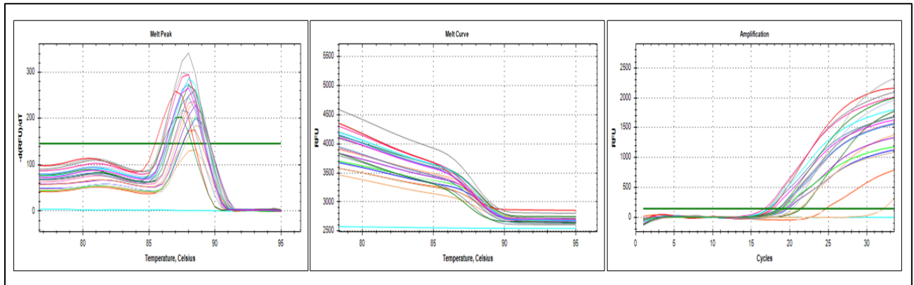
Fig S1: Melt peak, melt curve and amplification graphs of (A), PAL (B), CHS and (C) F3H generated in qRT-PCR.
