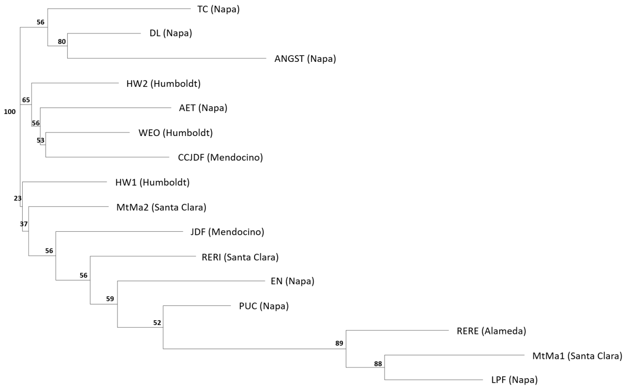
S5 Fig. Neighbour-joining tree of the 16 Californian reference populations represented by samples collected in 2017 (data set C). It is based on six cpSSR markers and Nei's genetic distance ([47] after [48]) with 1000 bootstraps. Numbers indicate bootstrap values in terms of percentage. County names of sampling sites are in brackets.
