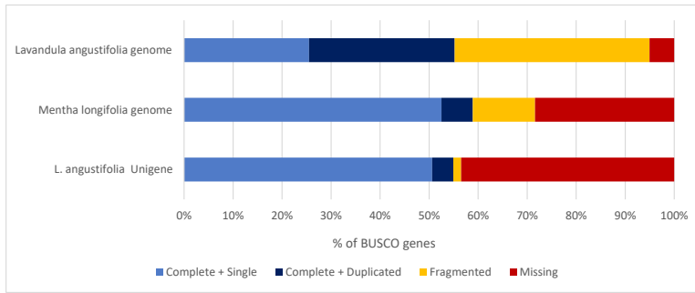
S2 Fig. Comparison of the completeness of lavender Unigene with the completeness of Lavandula angustifolia and Mentha longifolia genomes using BUSCO.
