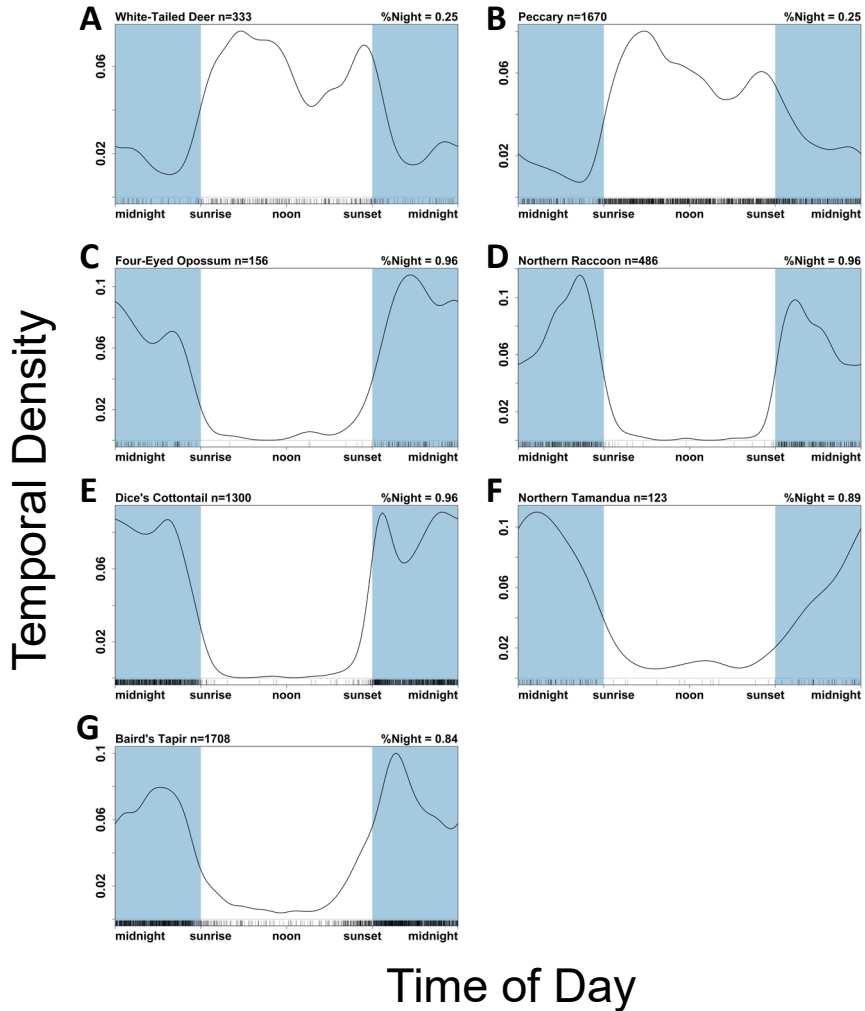
Supplementary Data SD7-2. Circadian activity density of 7 prey species based on all survey sites 2010-2019: (A) white-tailed deer, (B) collared peccary, (C) four-eyed opossum, (D) raccoon, (E) Dice's cottontail, (F) tamandua, and (G) Baird's tapir. Time of day is based on sun time. Sample size of independent records (n) and percent time active at night (%Night) are indicated on the top of each plot frame.
