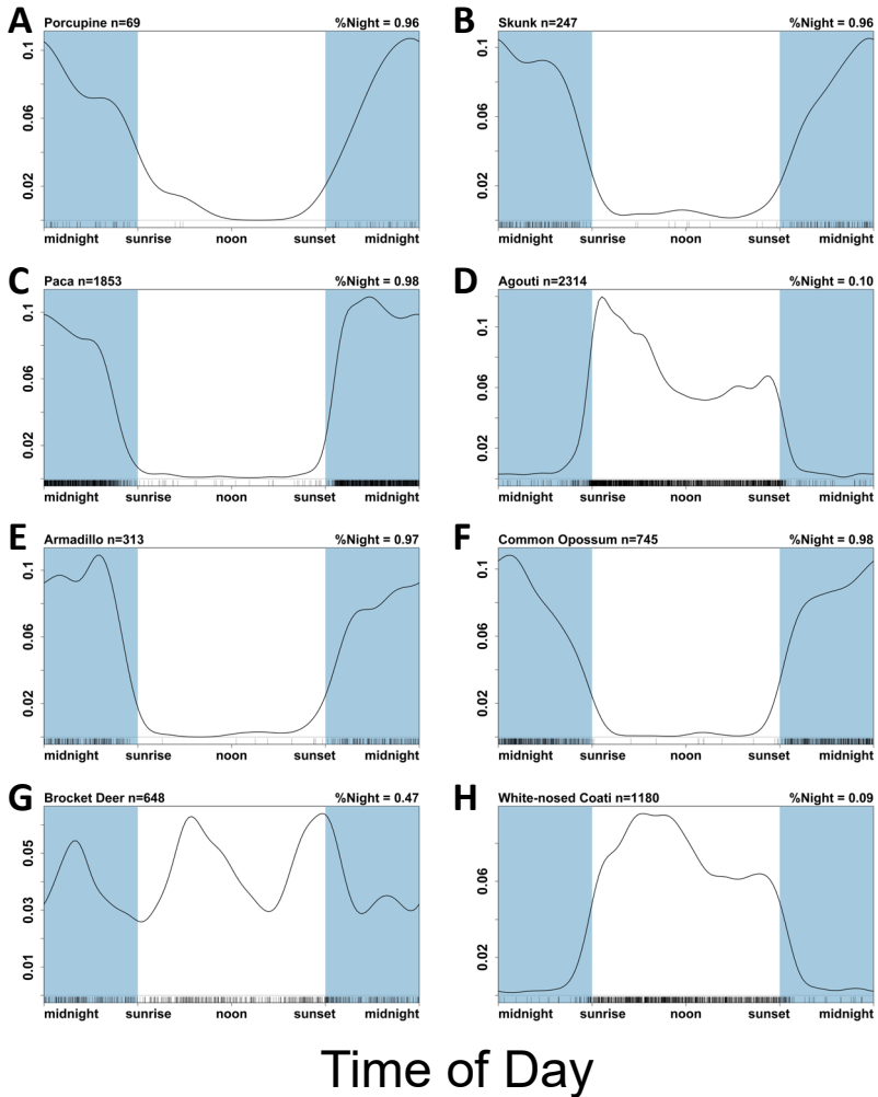
Supplementary Data SD7-1. Circadian activity density of 8 prey species based on all survey sites 2010-2019: (A) porcupine, (B) skunk, (C) paca, (D) agouti, (E) armadillo, (F) common opossum, (G) red brocket deer, and (H) coati. Time of day is based on sun time. Sample size of independent records (n) and percent time active at night (%Night) are indicated on the top of each plot frame.
