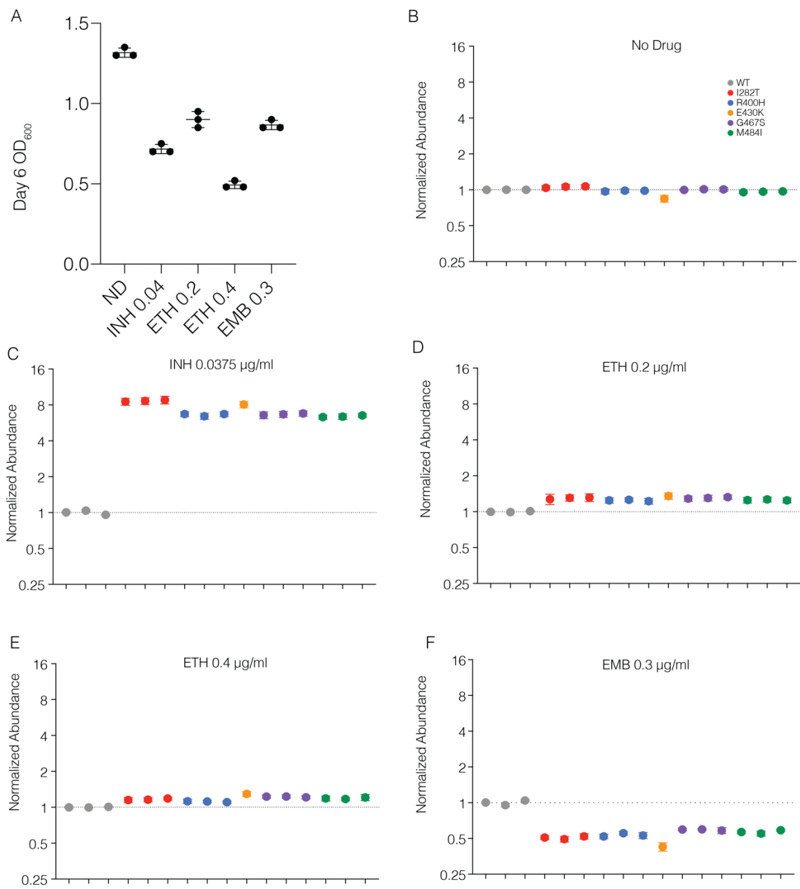
Figure S7. Competition of dnaA mutants during treatment with partially inhibitory concentrations of ethionamide (ETH) and ethambutol (EMB). INH is included as a positive control. (A) Final OD 600 of the bulk culture after 6 days of growth. Each dot represents an independent culture with the mean and standard deviation shown. (B-F) Relative abundance of each strain normalized to input library. Dots represent mean normalized abundance and bars show the standard deviation of three replicates.
