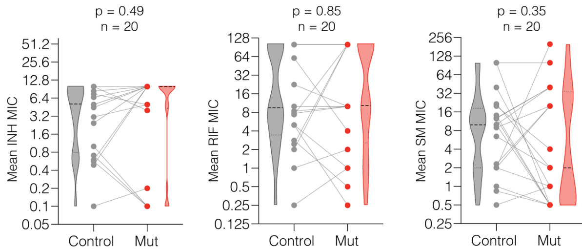
Figure S12. Comparison of the mean MIC of phylogenetic clades bearing any Rv0010c-Rv0011c mutation (red dots) with their nearest non-mutant neighbors (gray dots). Dashed line represents the median of the dataset. Gray lines between dots indicate each independent phylogenetic contrast. Difference in distribution tested by two-tailed Wilcoxon matched-pairs signed rank test.
