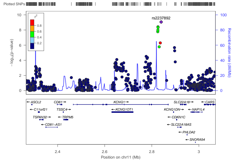
(a) T2D p-values
