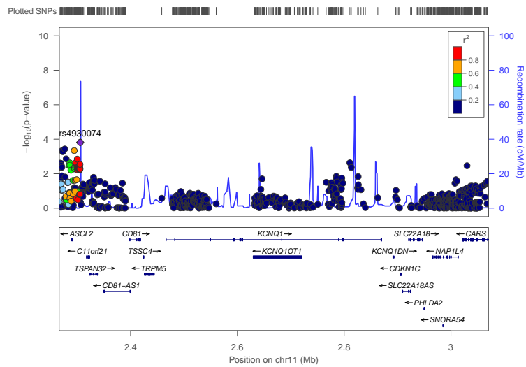
(c) PLACO p-values
