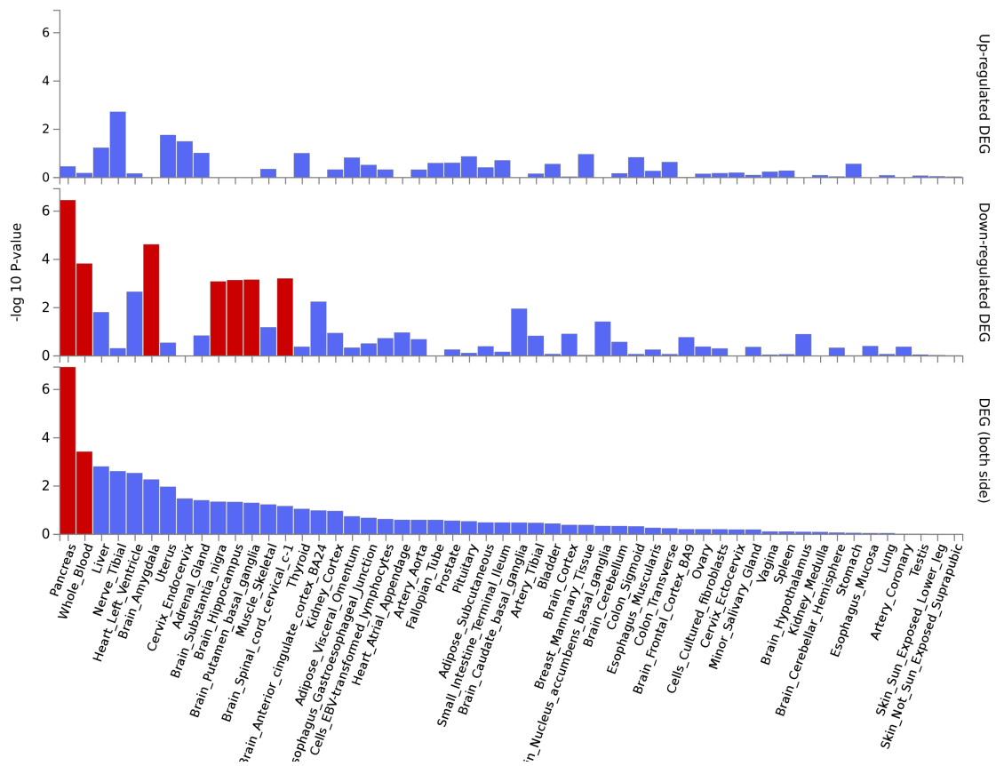
S10 Fig: Mapped genes (as done by FUMA) for the 43 pleiotropic loci detected by PLACO were tested against each of the Differentially Expressed Gene (DEG) sets pre-calculated from GTEx v8 tissue data from 53 tissue types.
