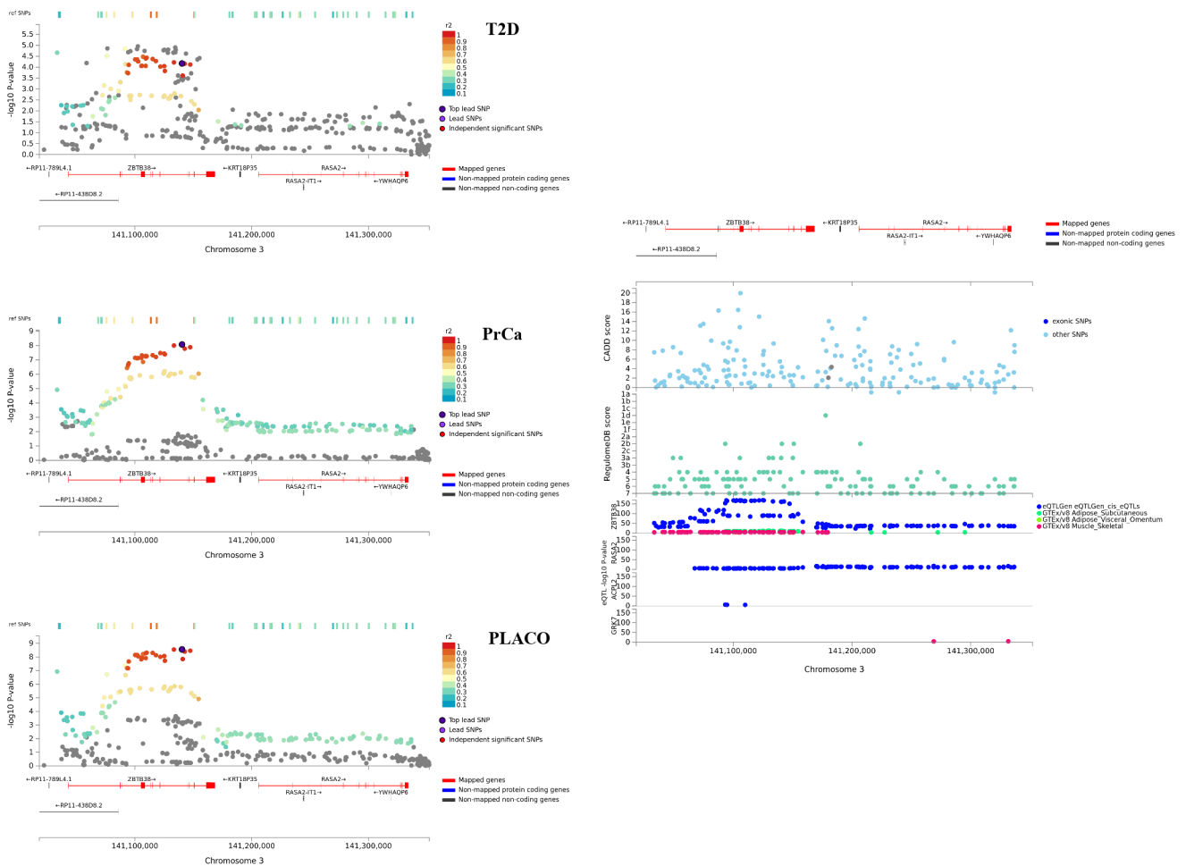
S11 Fig: Regional association plot of significant pleiotropic locus near ZBTB38 with annotations such as CADD scores, RegulomeDB scores, and cis eQTL association p-values from 6 tissues. Tissues considered are whole blood from eQTLGen Consortium; and adipose, liver, muscle-skeletal, pancreas, and prostate tissues from GTEx v8.
