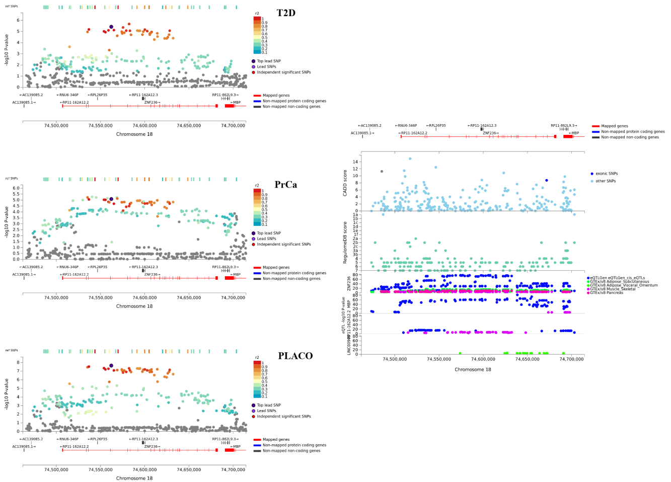
S16 Fig: Regional association plot of significant pleiotropic locus near ZNF236 with annotations such as CADD scores, RegulomeDB scores, and cis eQTL association p-values from 6 tissues. Tissues considered are whole blood from eQTLGen Consortium; and adipose, liver, muscle-skeletal, pancreas, and prostate tissues from GTEx v8.
