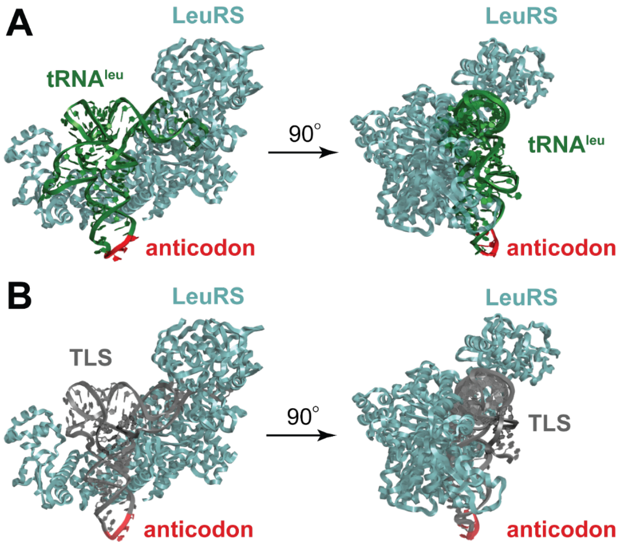
Supplemental Figure S4. The anticodon loop is recognized by Leucyl-tRNA synthetase (LeuRS). (A) Structure of tRNA Leu (green; anticodon nucleotides in red) in complex with LeuRS (blue) from Pyrococcus horikoshii , previously solved by X-ray crystallography (Fukunaga and Yokoyama 2005). (B) Modeling of the TYMV TLS (grey; anticodon nucleotides in red) (Colussi et al. 2014) with LeuRS (blue) from P. horikoshii .
