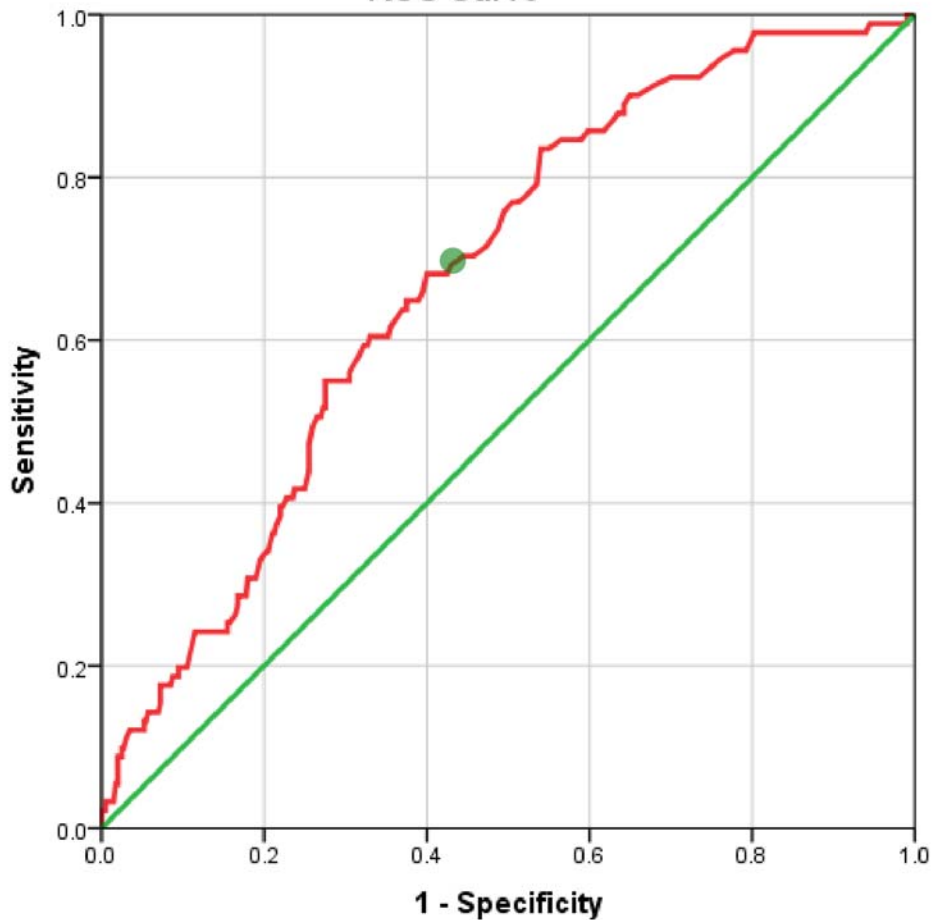
ROC Curve
