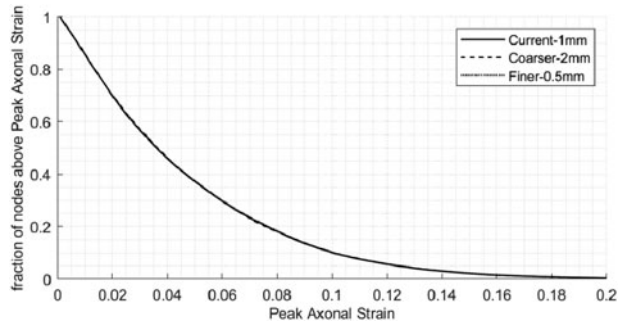
SUPPLEMENTARY FIG. S1. The axonal strain cumulative distribution curves extracted from the brain finite element model using fibers with 1mm (current, solid line), 2mm (coarser, dashed) and 0.5mm (finer, dotted) element sizes.
