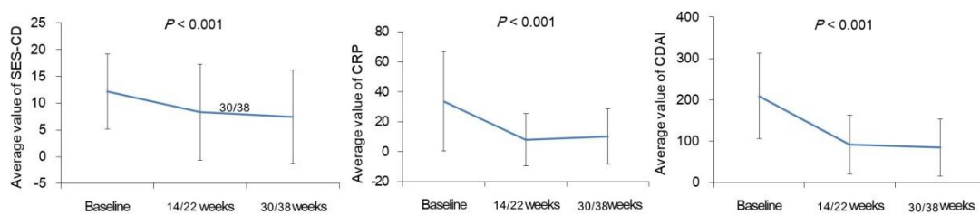
Supplemental Figure 1. Changes from baseline to 30/38 weeks in total SES-CD, CRP and CDAI in patients with CD.
