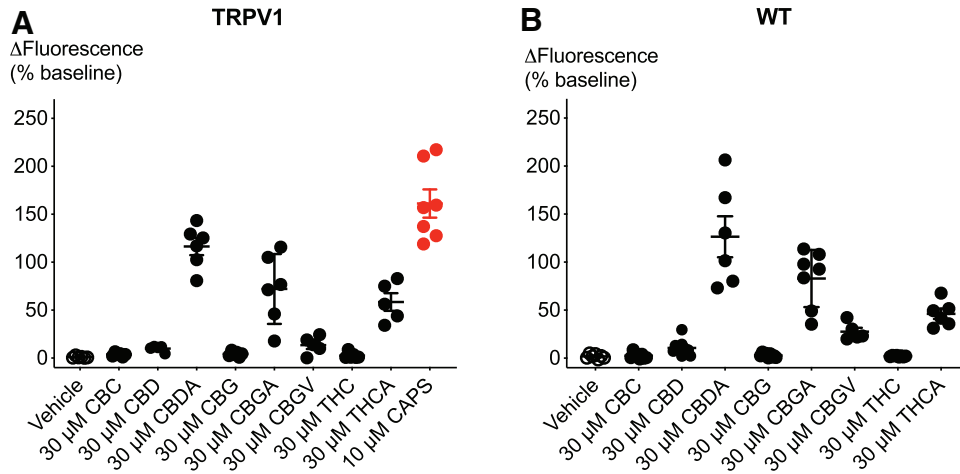
SUPPLEMENTARY FIG. S2. Effects of phytocannabinoids on hTRPV1 and WT cells. (A) Response of hTRPV1 cells to common phytocannabinoids. (B) CBDA, CBGA, CBGV, and THCA induce an increase in [Ca]_i in WT cells. Effects of phytocannabinoids are not significantly different between hTRPV1 and WT cells. Unpaired t -test. N > 5 , mean \pm SEM. CBDA, cannabidiolic acid; CBGA, cannabigerolic acid; CBGV, cannabigerovarin; hTRPA1, human transient receptor potential ankyrin 1; hTRPV1, human transient receptor potential vanilloid 1; THCA, tetrahydrocannabinolic acid.
