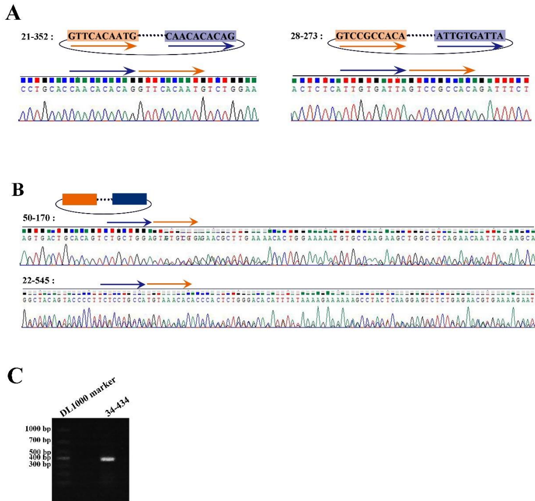
Supplementary Figure 1. Supplementary figure. (A) Sanger sequencing of 21-352 and 28-273 confirming the back-splicing junction in PCR products. (B) Sanger sequencing result of 50-170 and 22-545. (C) Amplification result of 34-434 using divergent PCR primers
