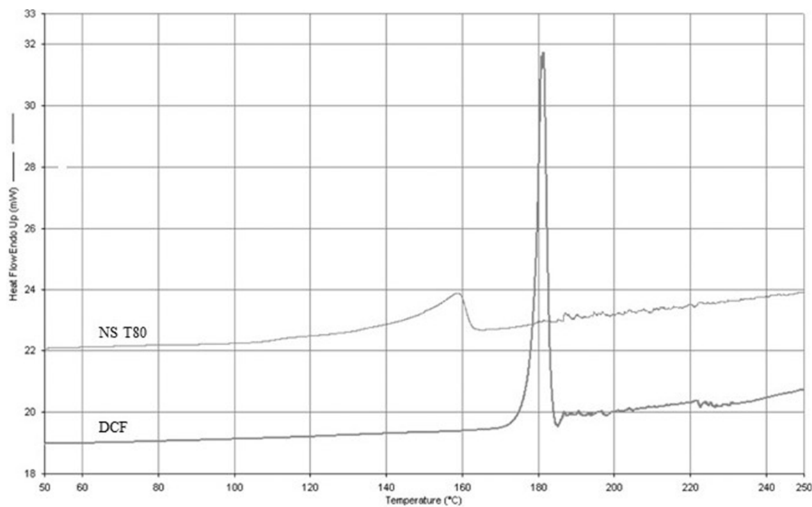
Figure S1. DSC thermograms of bulk DCF and DCF nanocrystals (NS T80).
