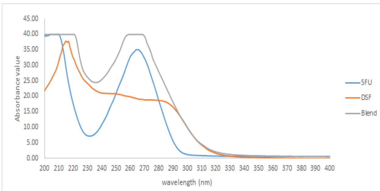
Figure S1. Scan of UV spectrum of 5-FU, DSF and as a blend from 200 to 400 nm.
