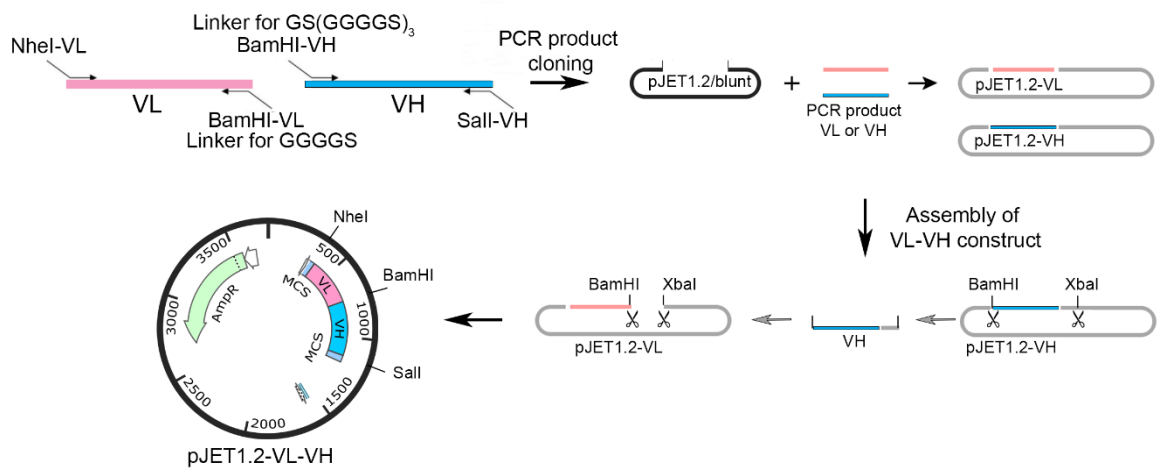
Figure S1. Schematic representation of the construction of expression vector for 14D6-derived scFv.
