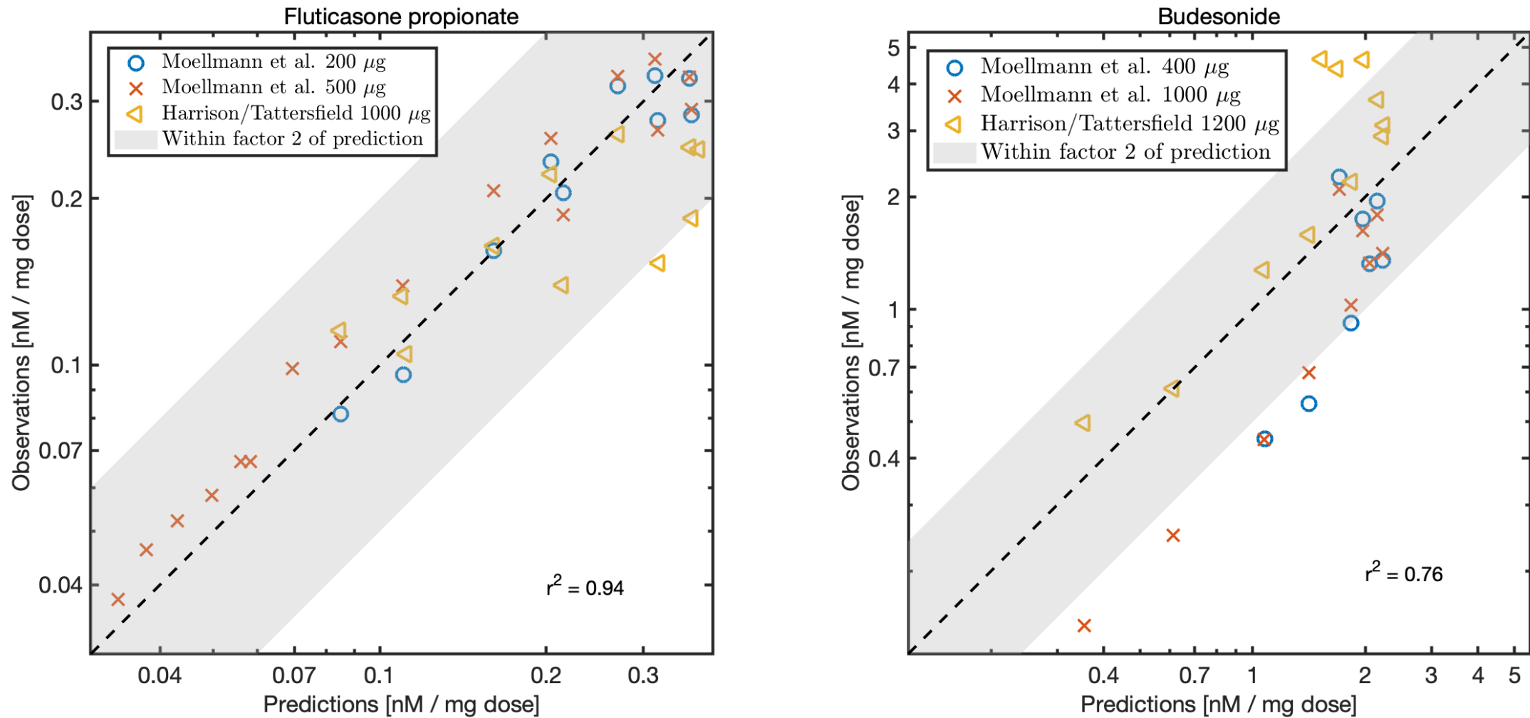
S5 Fig. Goodness-of-fit for pharmacokinetic data in healthy volunteers.
