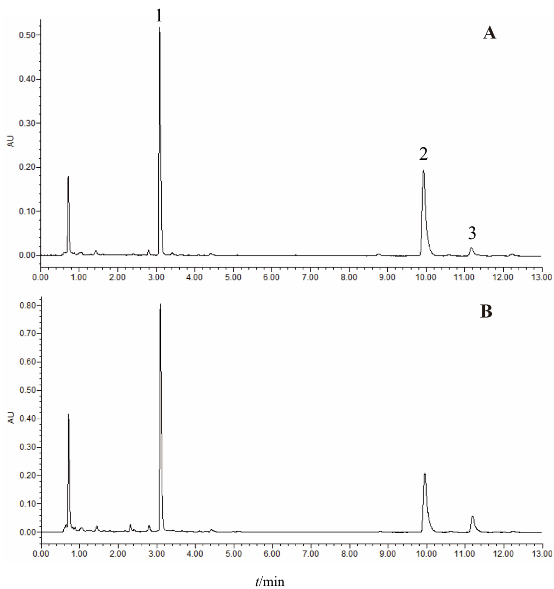
Figure S1| UPLC chromatograms of PS decoctions at 254 nm wavelength: A-CPS, B-SPS 1—geniposidic acid, 2—verbascoside, 3—isoverbascoside
