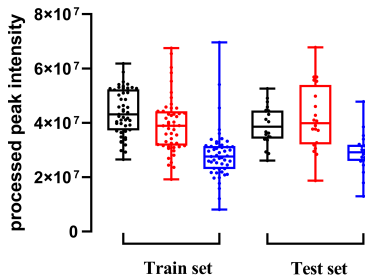
Linoleic Acid
