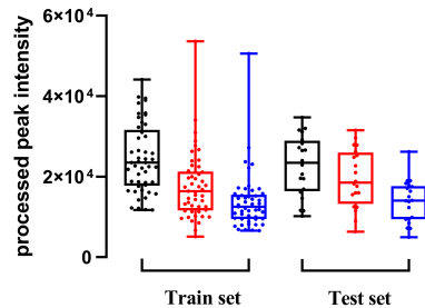
Eicosadienoic Acid
