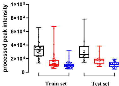
Dihomo- \gamma -Linolenic Acid
