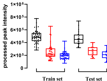
Arachidonic Acid
