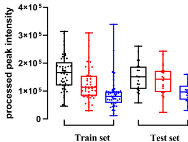
\gamma -Linolenic Acid
